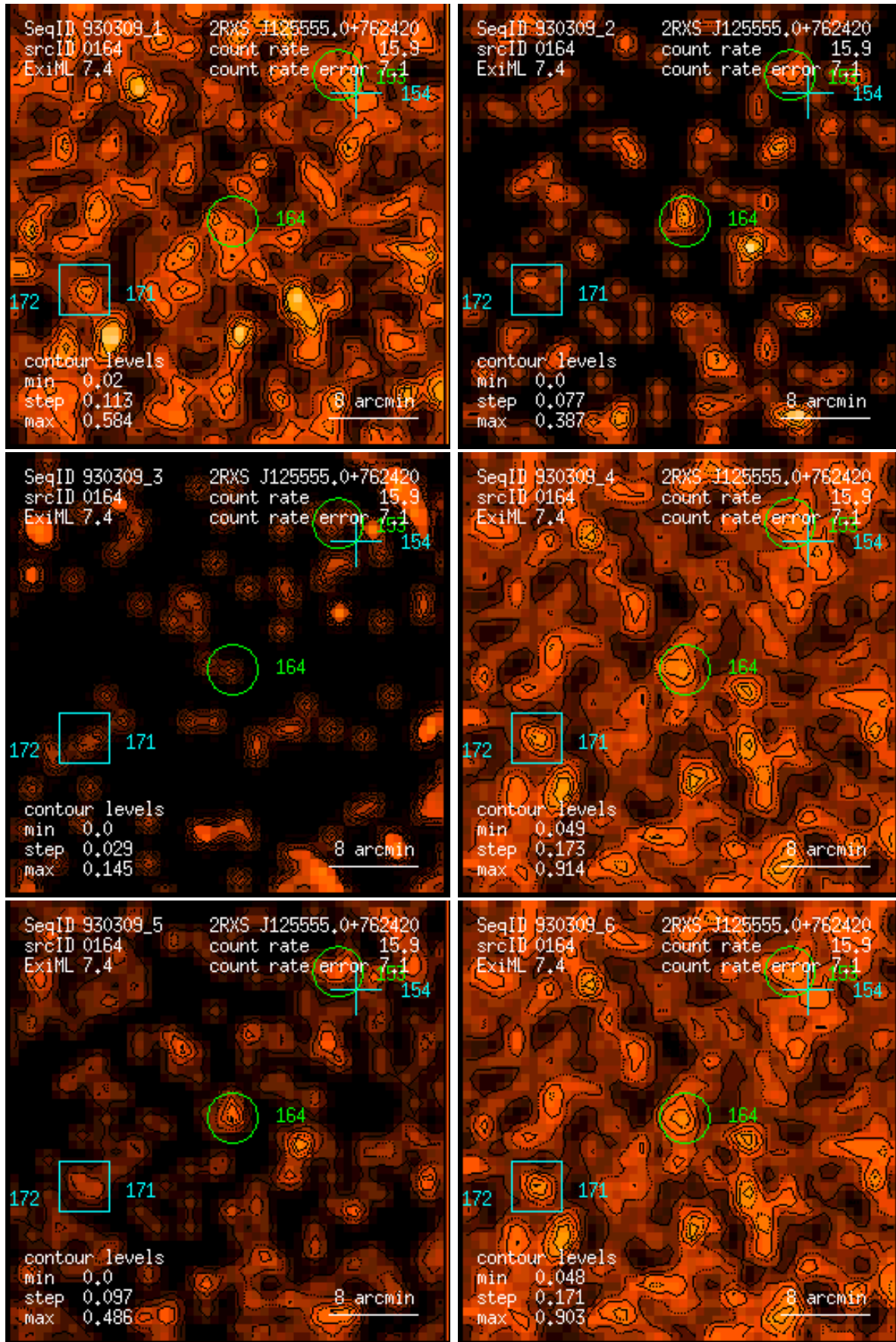
Figure 164: RASS 930309: detection 0164: band rate images, Gaussian filter: (1) PSPC channels 11 – 41, (2) 52 – 90, (3) 91 – 201, (4) 11 – 235, (5) 52 – 201, (6) 11 – 201. Broad band rates in counts/ks. Band rate contour levels in counts/ks/arcmin 2 .
