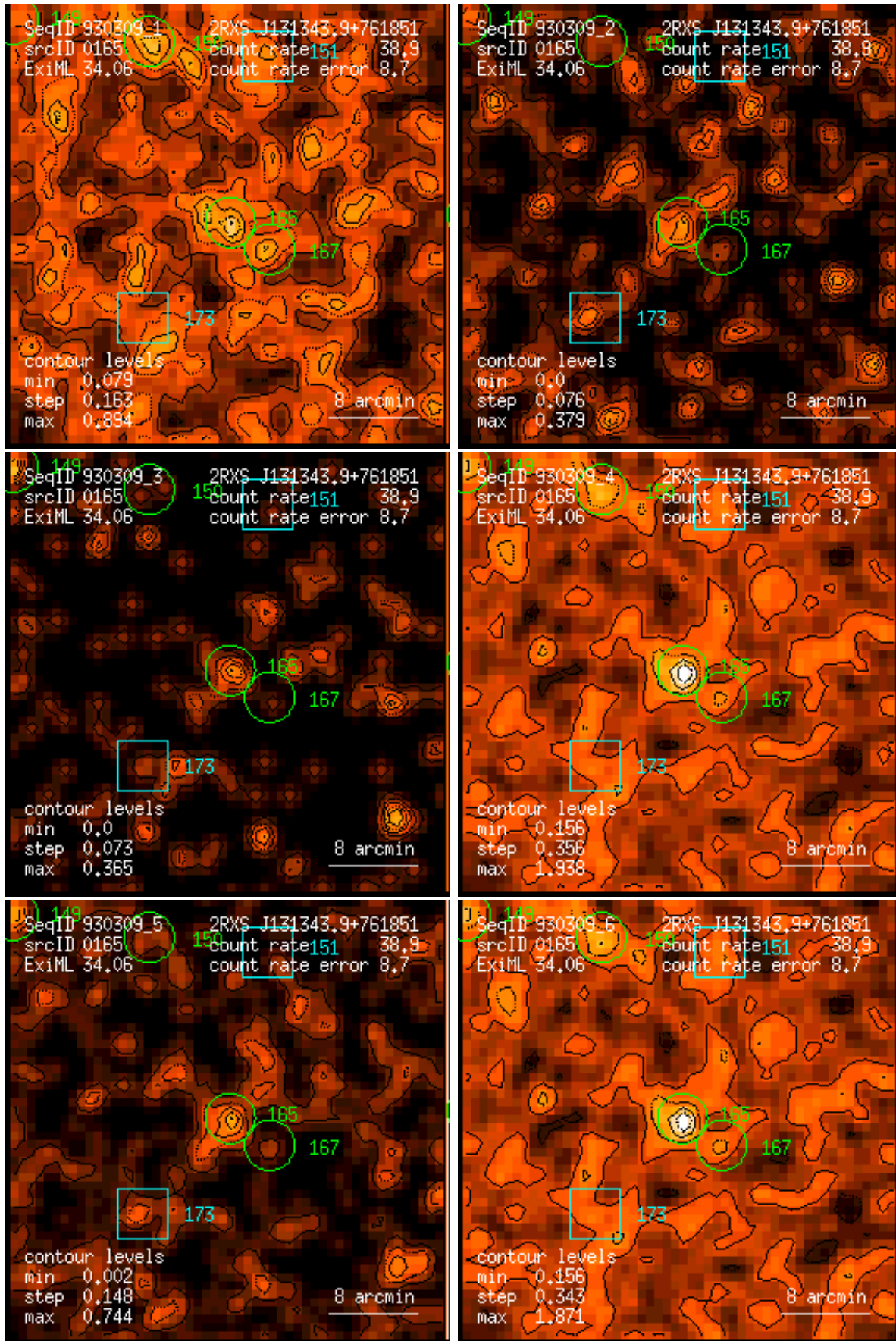
Figure 165: RASS 930309: detection 0165: band rate images, Gaussian filter: (1) PSPC channels 11 – 41, (2) 52 – 90, (3) 91 – 201, (4) 11 – 235, (5) 52 – 201, (6) 11 – 201. Broad band rates in counts/ks. Band rate contour levels in counts/ks/arcmin 2 .
