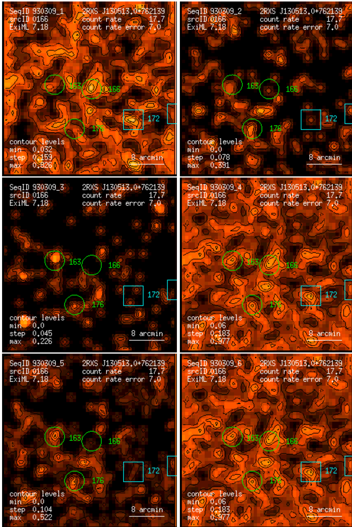
Figure 166: RASS 930309: detection 0166: band rate images, Gaussian filter: (1) PSPC channels 11 – 41, (2) 52 – 90, (3) 91 – 201, (4) 11 – 235, (5) 52 – 201, (6) 11 – 201. Broad band rates in counts/ks. Band rate contour levels in counts/ks/arcmin 2 .
