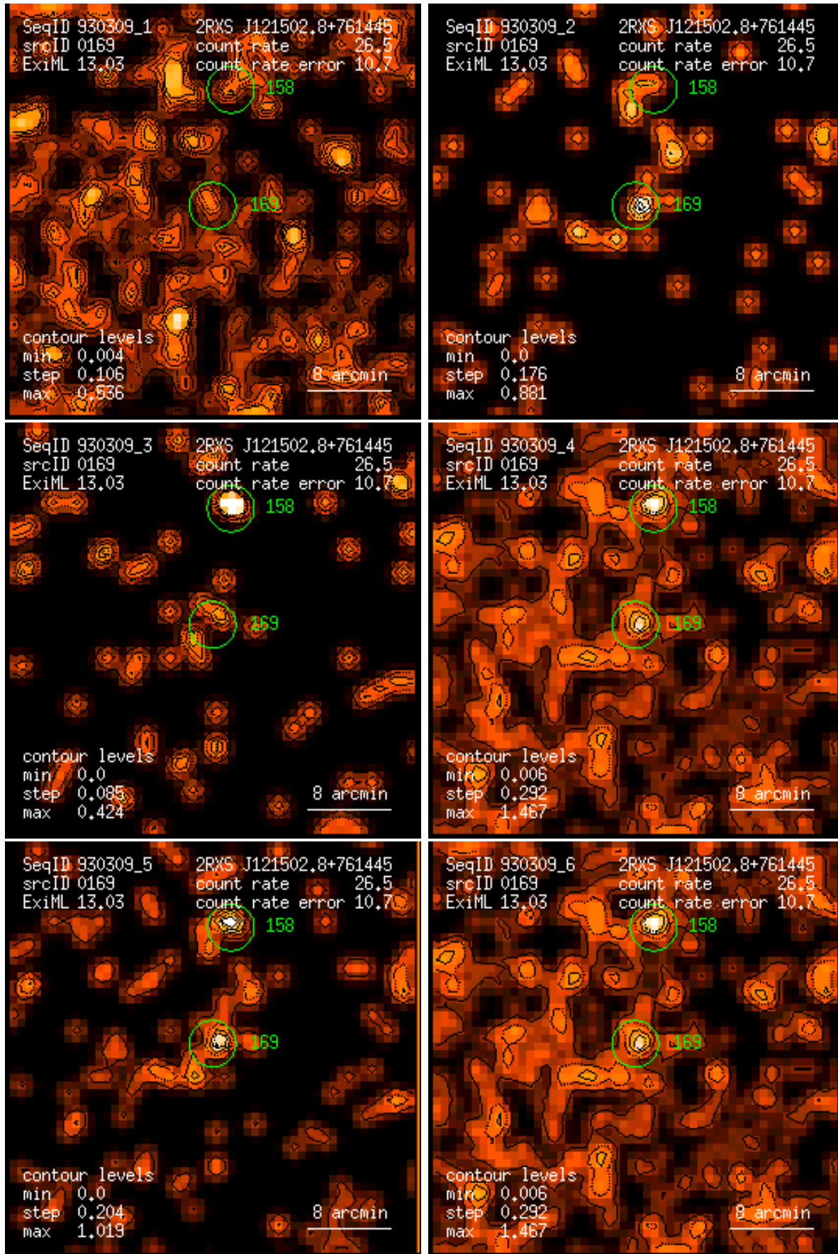
Figure 169: RASS 930309: detection 0169: band rate images, Gaussian filter: (1) PSPC channels 11 – 41, (2) 52 – 90, (3) 91 – 201, (4) 11 – 235, (5) 52 – 201, (6) 11 – 201. Broad band rates in counts/ks. Band rate contour levels in counts/ks/arcmin 2 .
