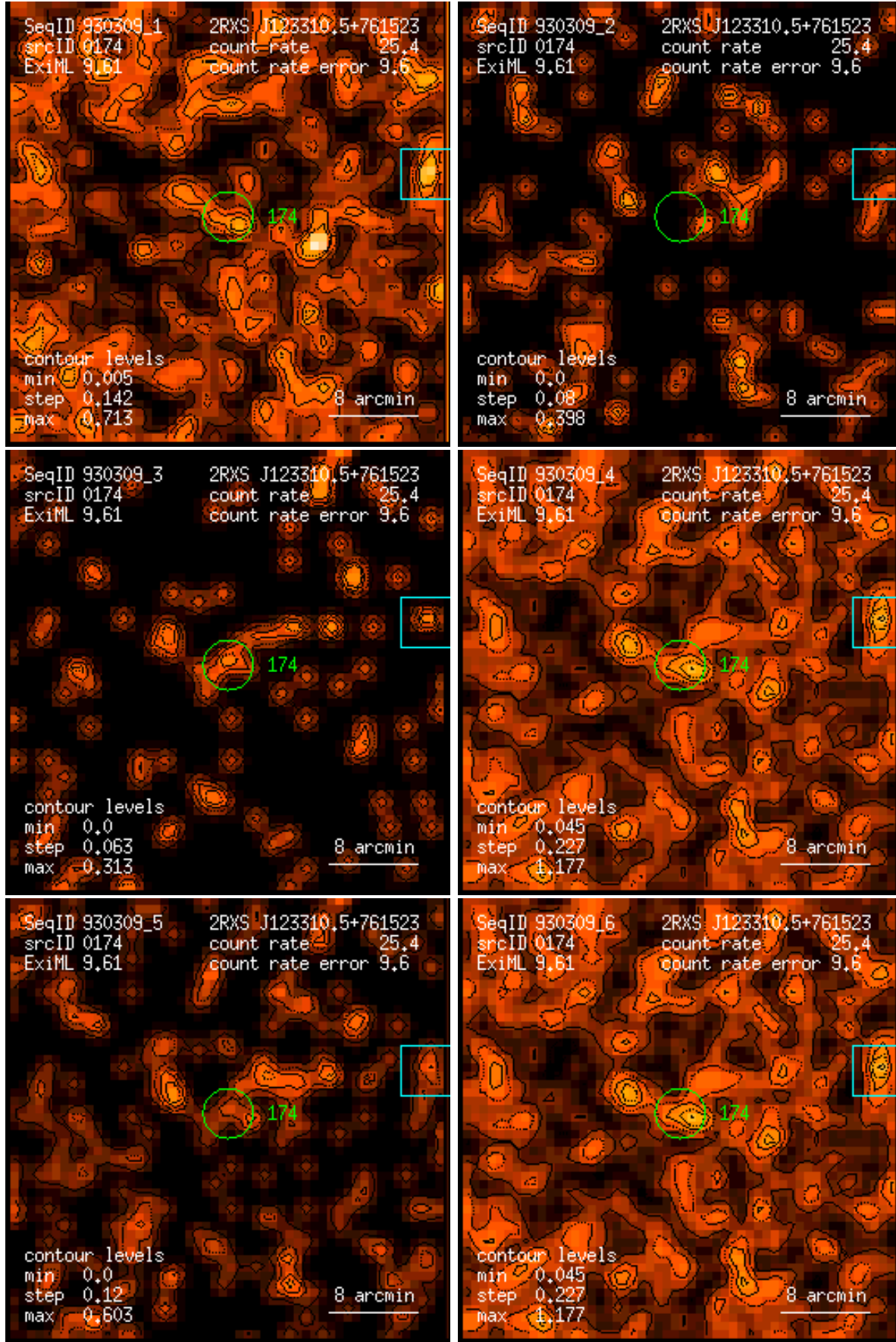
Figure 174: RASS 930309: detection 0174: band rate images, Gaussian filter: (1) PSPC channels 11 – 41, (2) 52 – 90, (3) 91 – 201, (4) 11 – 235, (5) 52 – 201, (6) 11 – 201. Broad band rates in counts/ks. Band rate contour levels in counts/ks/arcmin 2 .
