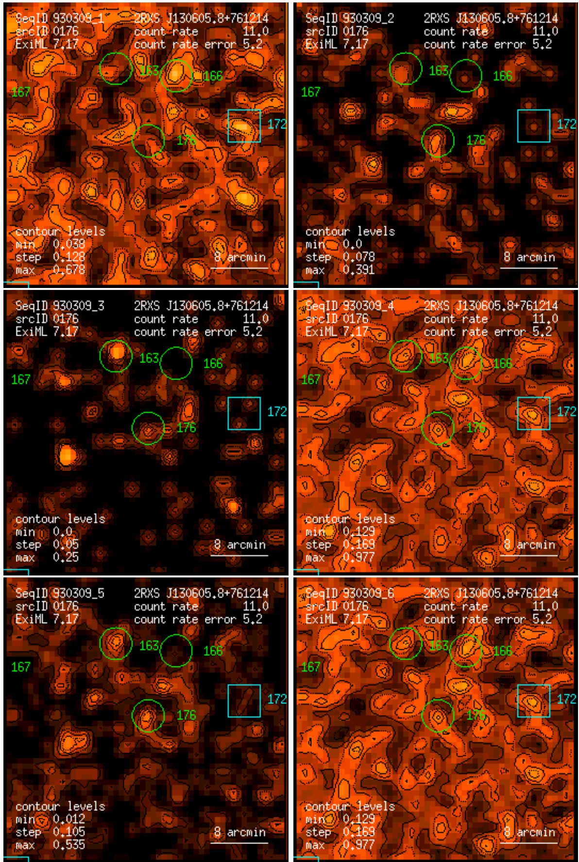
Figure 176: RASS 930309: detection 0176: band rate images, Gaussian filter: (1) PSPC channels 11 – 41, (2) 52 – 90, (3) 91 – 201, (4) 11 – 235, (5) 52 – 201, (6) 11 – 201. Broad band rates in counts/ks. Band rate contour levels in counts/ks/arcmin 2 .
