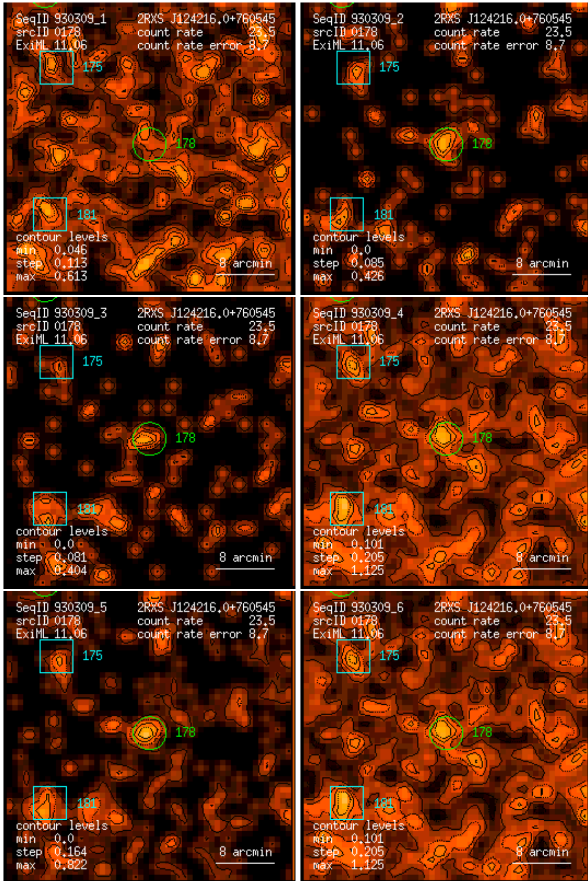
Figure 178: RASS 930309: detection 0178: band rate images, Gaussian filter: (1) PSPC channels 11 – 41, (2) 52 – 90, (3) 91 – 201, (4) 11 – 235, (5) 52 – 201, (6) 11 – 201. Broad band rates in counts/ks. Band rate contour levels in counts/ks/arcmin 2 .
