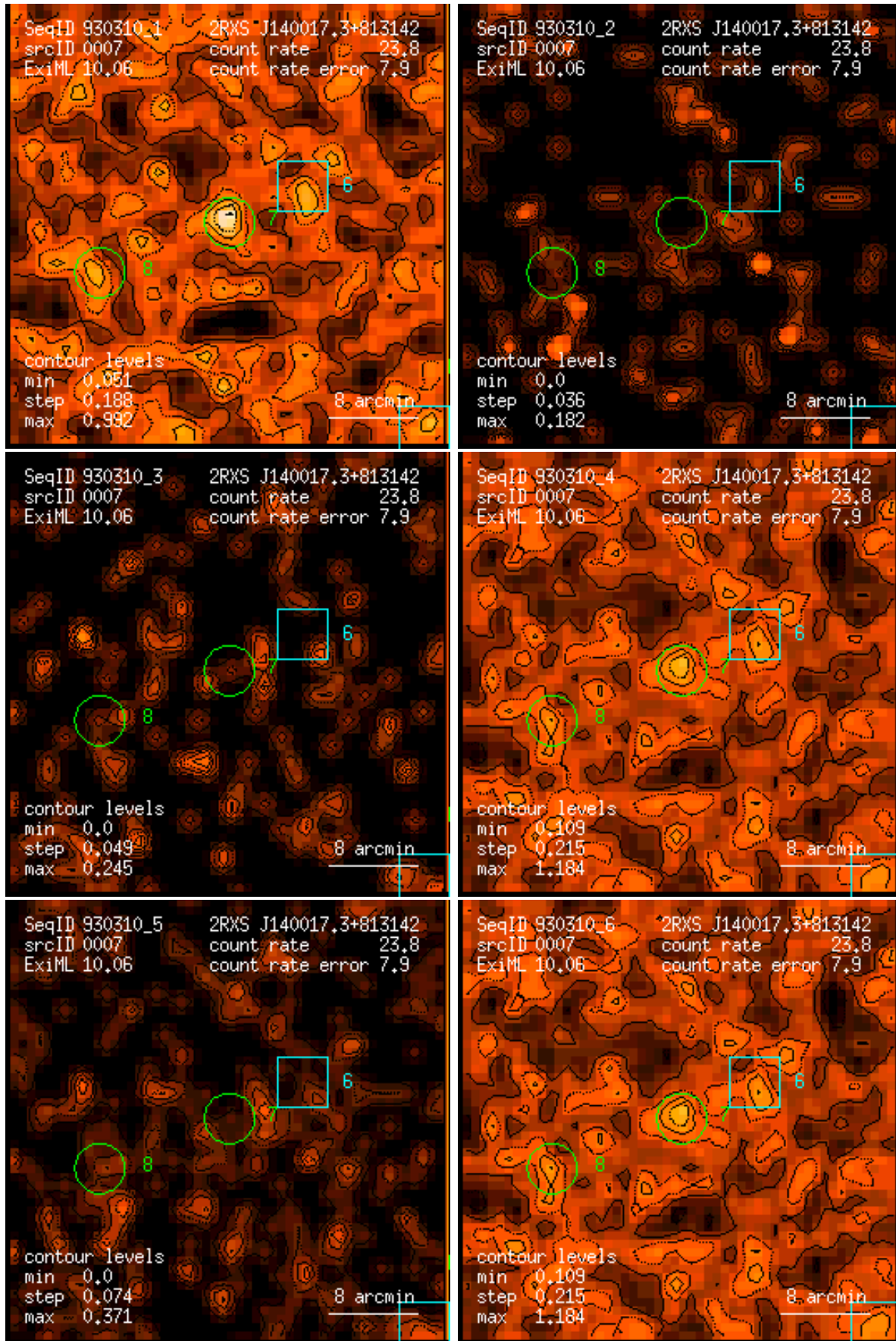
Figure 7: RASS 930310: detection 0007: band rate images, Gaussian filter: (1) PSPC channels 11 – 41, (2) 52 – 90, (3) 91 – 201, (4) 11 – 235, (5) 52 – 201, (6) 11 – 201. Broad band rates in counts/ks. Band rate contour levels in counts/ks/arcmin 2 .
