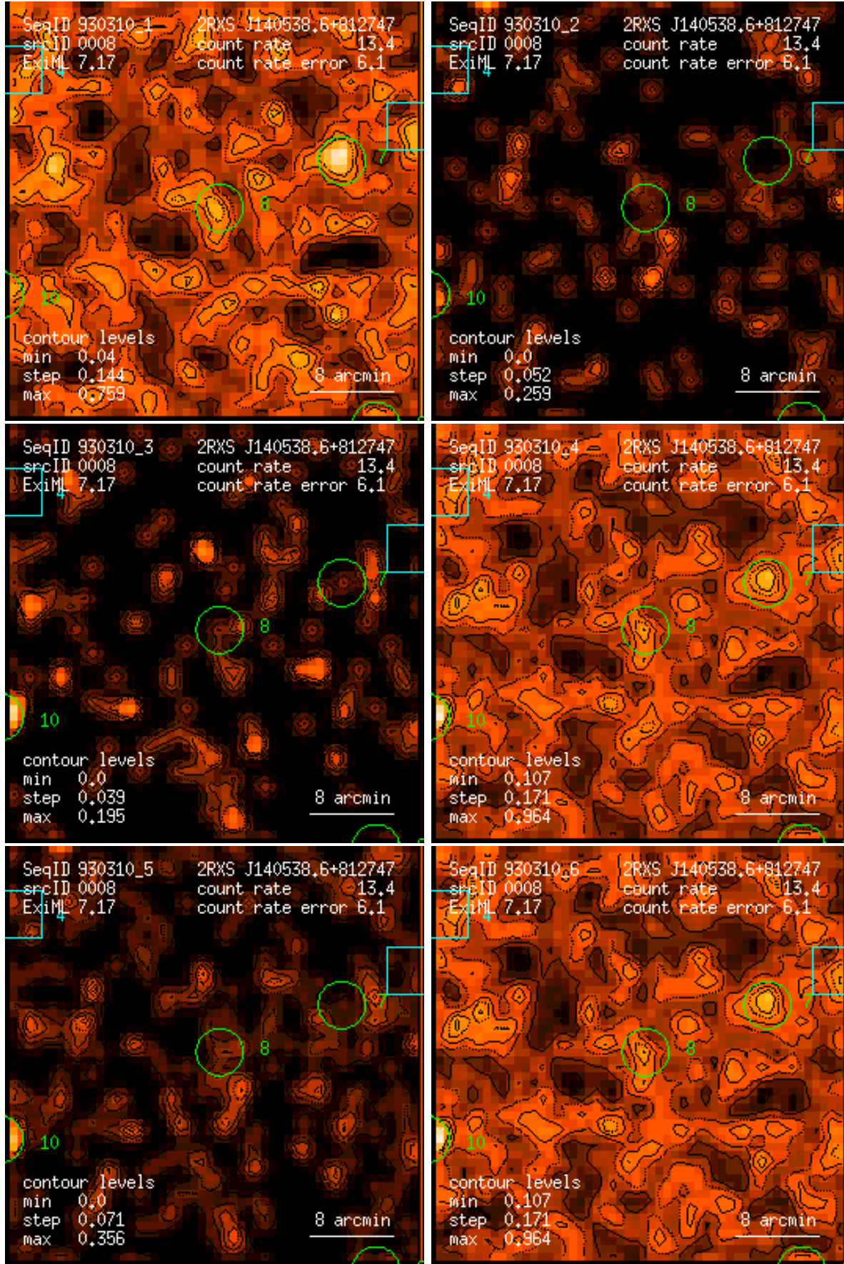
Figure 8: RASS 930310: detection 0008: band rate images, Gaussian filter: (1) PSPC channels 11 – 41, (2) 52 – 90, (3) 91 – 201, (4) 11 – 235, (5) 52 – 201, (6) 11 – 201. Broad band rates in counts/ks. Band rate contour levels in counts/ks/arcmin 2 .
