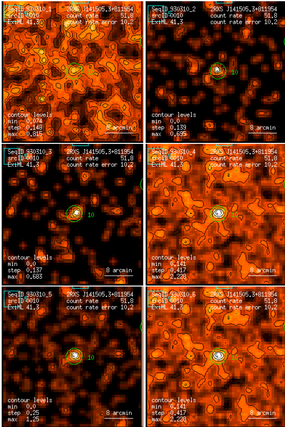
Figure 10: RASS 930310: detection 0010: band rate images, Gaussian filter: (1) PSPC channels 11 – 41, (2) 52 – 90, (3) 91 – 201, (4) 11 – 235, (5) 52 – 201, (6) 11 – 201. Broad band rates in counts/ks. Band rate contour levels in counts/ks/arcmin 2 .
