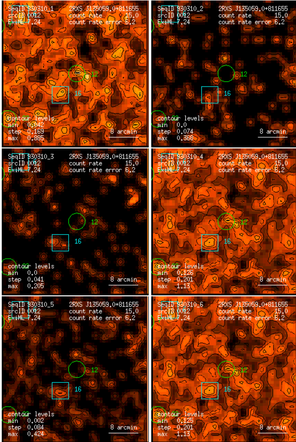
Figure 12: RASS 930310: detection 0012: band rate images, Gaussian filter: (1) PSPC channels 11 – 41, (2) 52 – 90, (3) 91 – 201, (4) 11 – 235, (5) 52 – 201, (6) 11 – 201. Broad band rates in counts/ks. Band rate contour levels in counts/ks/arcmin 2 .
