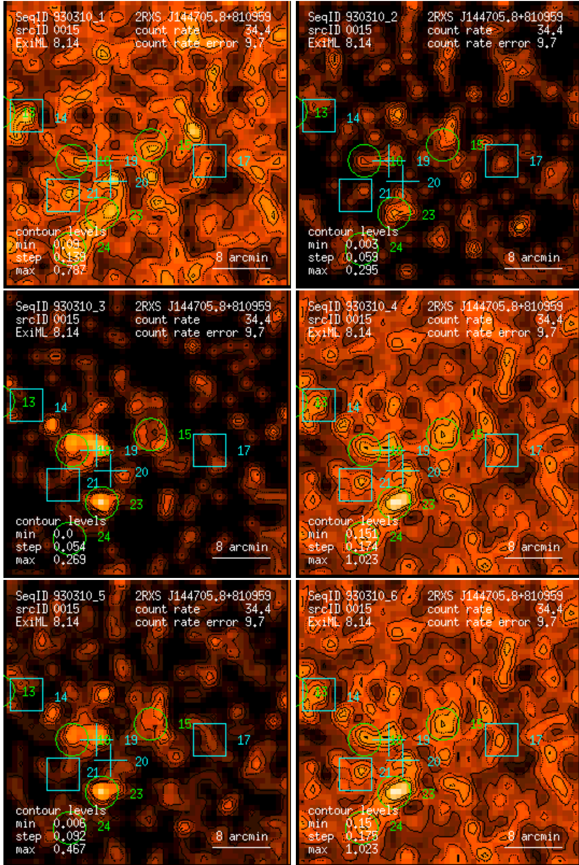
Figure 15: RASS 930310: detection 0015: band rate images, Gaussian filter: (1) PSPC channels 11 – 41, (2) 52 – 90, (3) 91 – 201, (4) 11 – 235, (5) 52 – 201, (6) 11 – 201. Broad band rates in counts/ks. Band rate contour levels in counts/ks/arcmin 2 .
