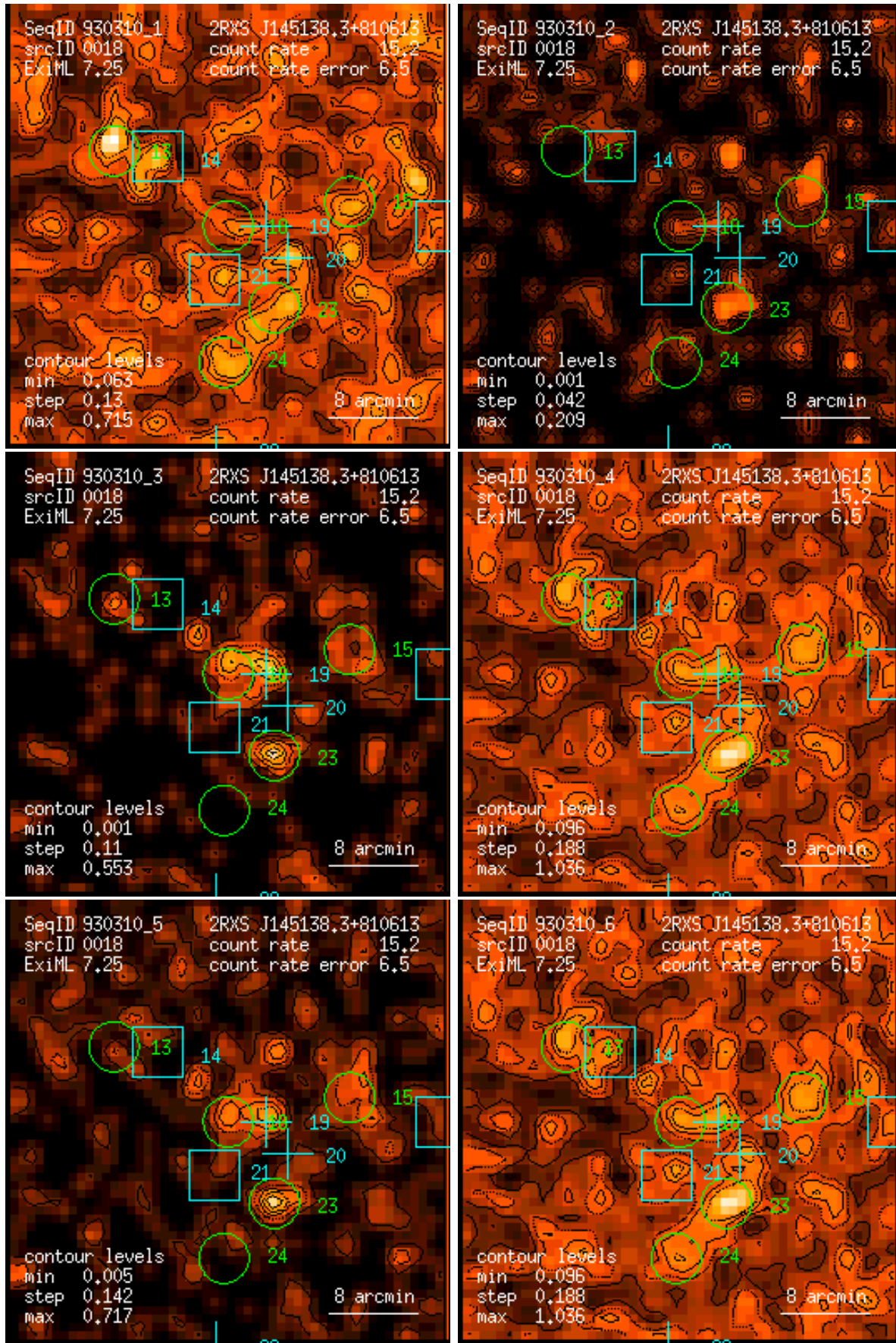
Figure 18: RASS 930310: detection 0018: band rate images, Gaussian filter: (1) PSPC channels 11 – 41, (2) 52 – 90, (3) 91 – 201, (4) 11 – 235, (5) 52 – 201, (6) 11 – 201. Broad band rates in counts/ks. Band rate contour levels in counts/ks/arcmin 2 .
