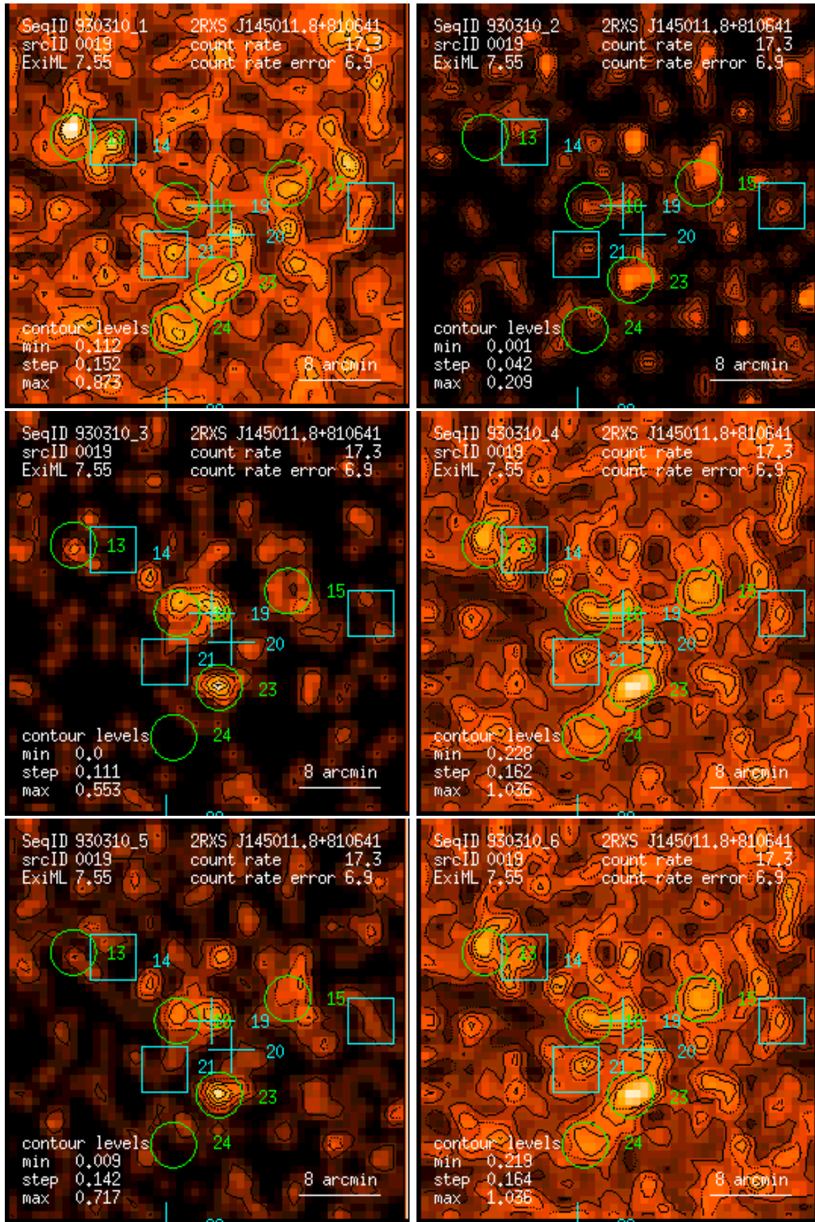
Figure 19: RASS 930310: detection 0019: band rate images, Gaussian filter: (1) PSPC channels 11 – 41, (2) 52 – 90, (3) 91 – 201, (4) 11 – 235, (5) 52 – 201, (6) 11 – 201. Broad band rates in counts/ks. Band rate contour levels in counts/ks/arcmin 2 .
