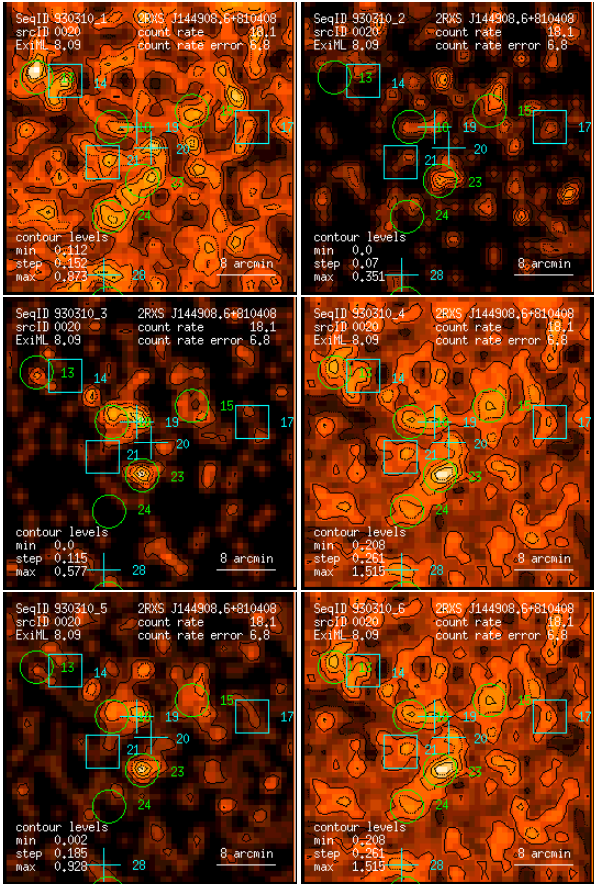
Figure 20: RASS 930310: detection 0020: band rate images, Gaussian filter: (1) PSPC channels 11 – 41, (2) 52 – 90, (3) 91 – 201, (4) 11 – 235, (5) 52 – 201, (6) 11 – 201. Broad band rates in counts/ks. Band rate contour levels in counts/ks/arcmin 2 .
