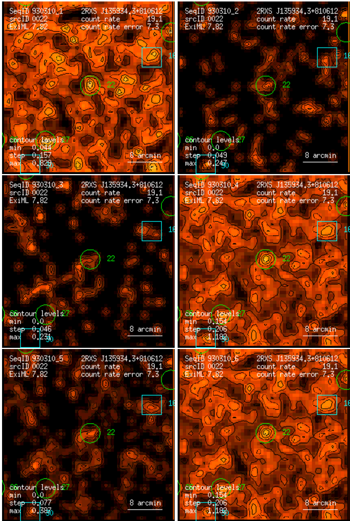
Figure 22: RASS 930310: detection 0022: band rate images, Gaussian filter: (1) PSPC channels 11 – 41, (2) 52 – 90, (3) 91 – 201, (4) 11 – 235, (5) 52 – 201, (6) 11 – 201. Broad band rates in counts/ks. Band rate contour levels in counts/ks/arcmin 2 .
