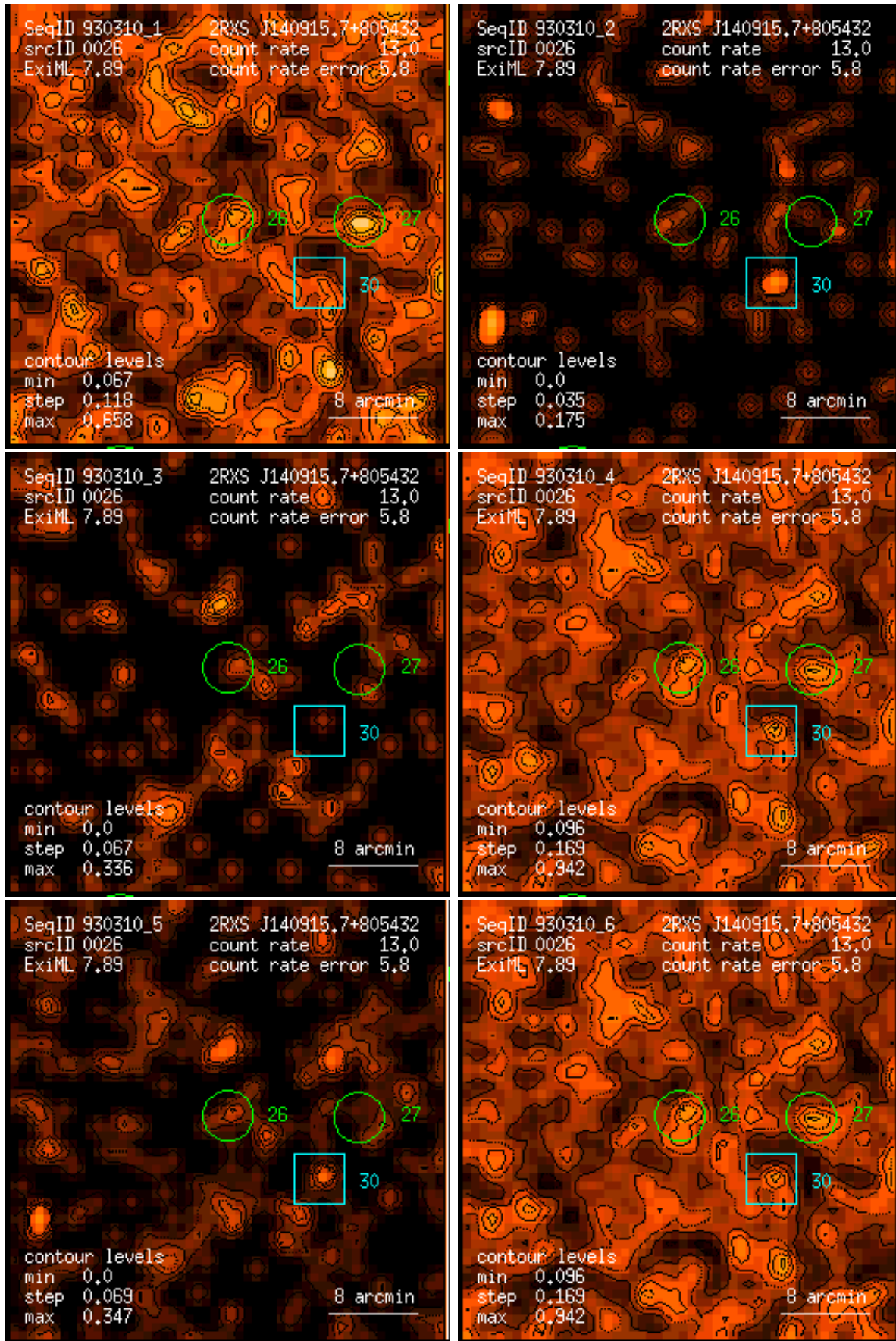
Figure 26: RASS 930310: detection 0026: band rate images, Gaussian filter: (1) PSPC channels 11 – 41, (2) 52 – 90, (3) 91 – 201, (4) 11 – 235, (5) 52 – 201, (6) 11 – 201. Broad band rates in counts/ks. Band rate contour levels in counts/ks/arcmin 2 .
