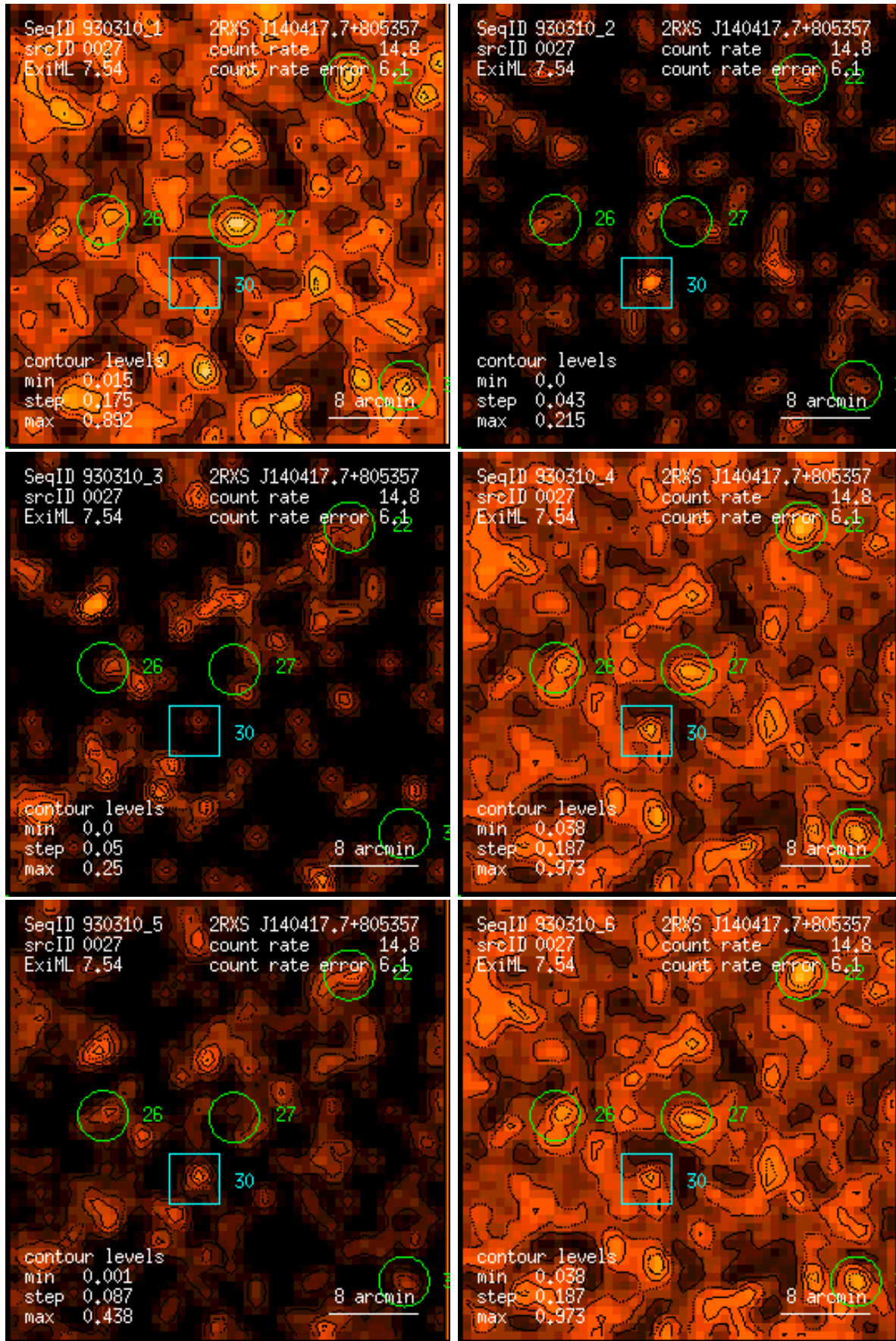
Figure 27: RASS 930310: detection 0027: band rate images, Gaussian filter: (1) PSPC channels 11 – 41, (2) 52 – 90, (3) 91 – 201, (4) 11 – 235, (5) 52 – 201, (6) 11 – 201. Broad band rates in counts/ks. Band rate contour levels in counts/ks/arcmin 2 .
