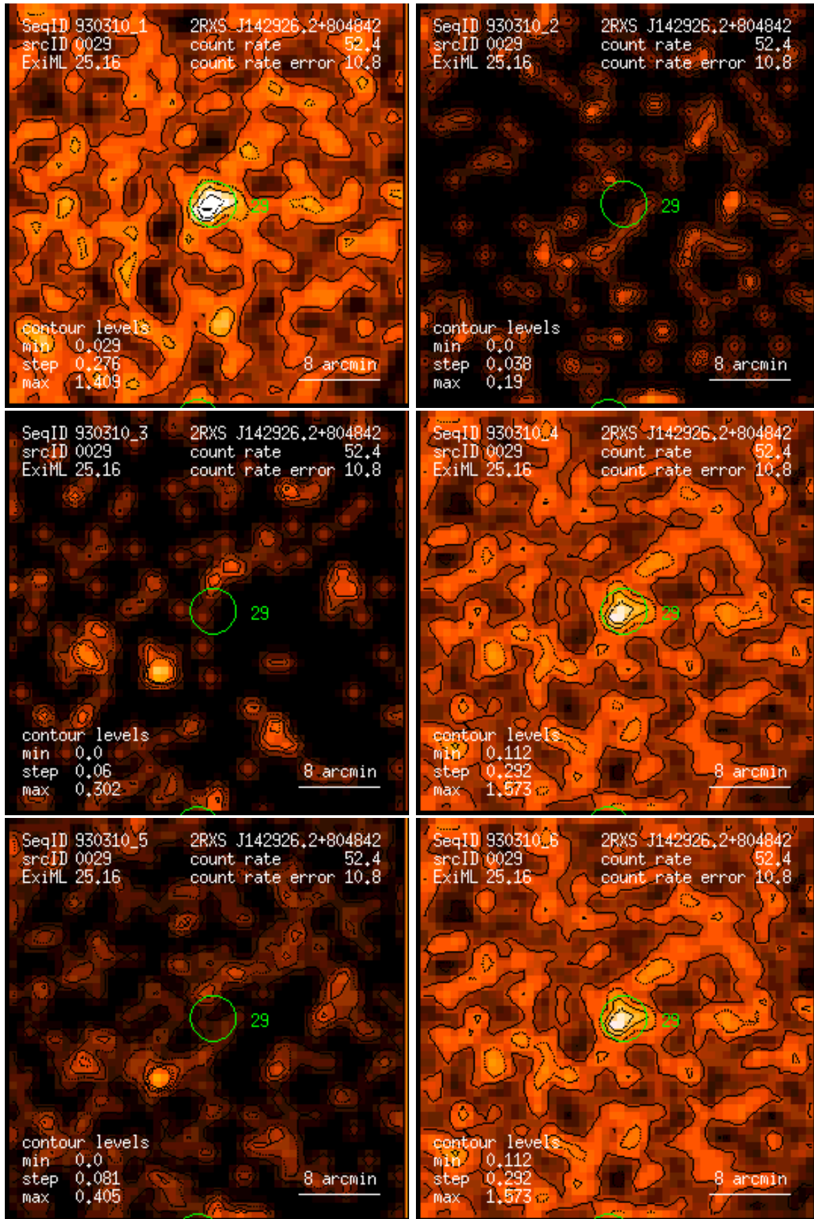
Figure 29: RASS 930310: detection 0029: band rate images, Gaussian filter: (1) PSPC channels 11 – 41, (2) 52 – 90, (3) 91 – 201, (4) 11 – 235, (5) 52 – 201, (6) 11 – 201. Broad band rates in counts/ks. Band rate contour levels in counts/ks/arcmin 2 .
