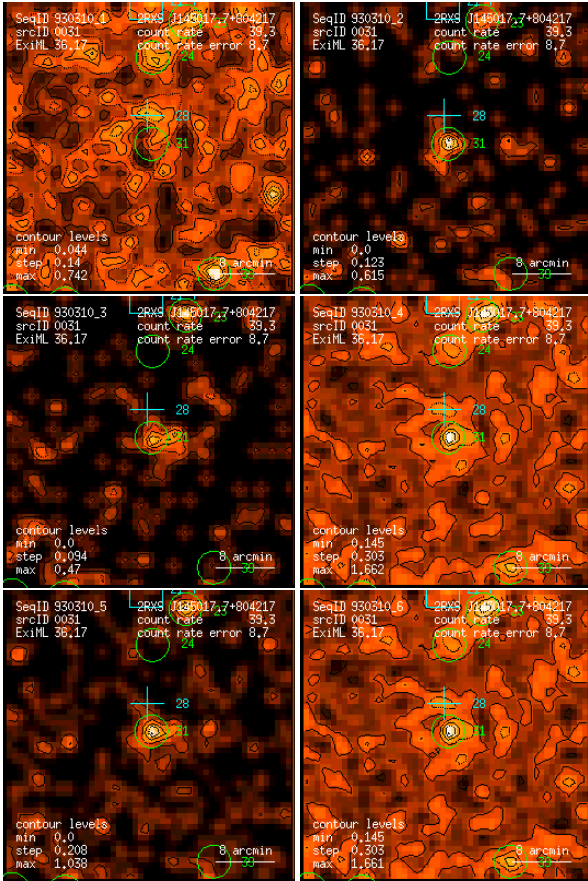
Figure 31: RASS 930310: detection 0031: band rate images, Gaussian filter: (1) PSPC channels 11 – 41, (2) 52 – 90, (3) 91 – 201, (4) 11 – 235, (5) 52 – 201, (6) 11 – 201. Broad band rates in counts/ks. Band rate contour levels in counts/ks/arcmin 2 .
