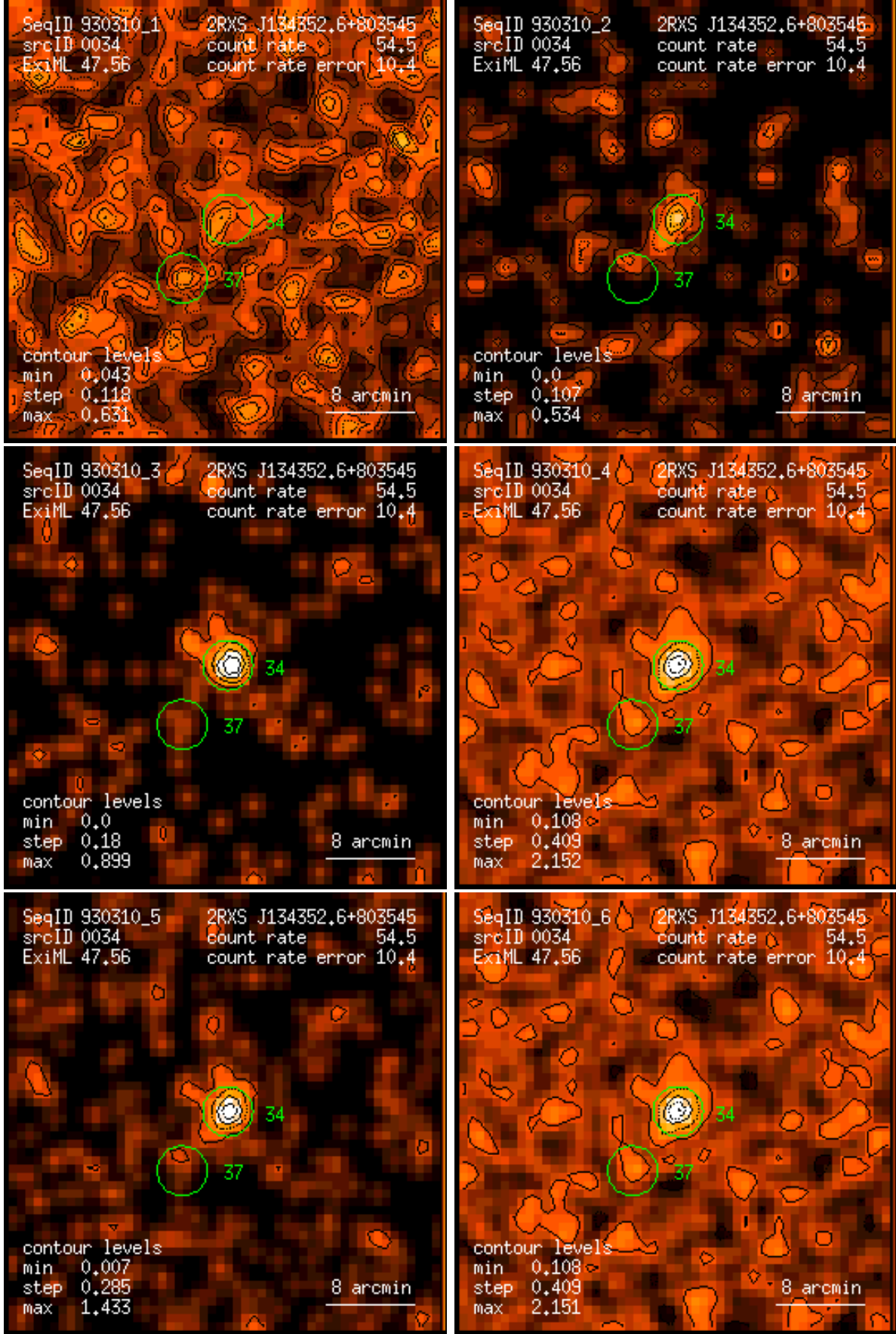
Figure 34: RASS 930310: detection 0034: band rate images, Gaussian filter: (1) PSPC channels 11 – 41, (2) 52 – 90, (3) 91 – 201, (4) 11 – 235, (5) 52 – 201, (6) 11 – 201. Broad band rates in counts/ks. Band rate contour levels in counts/ks/arcmin 2 .
