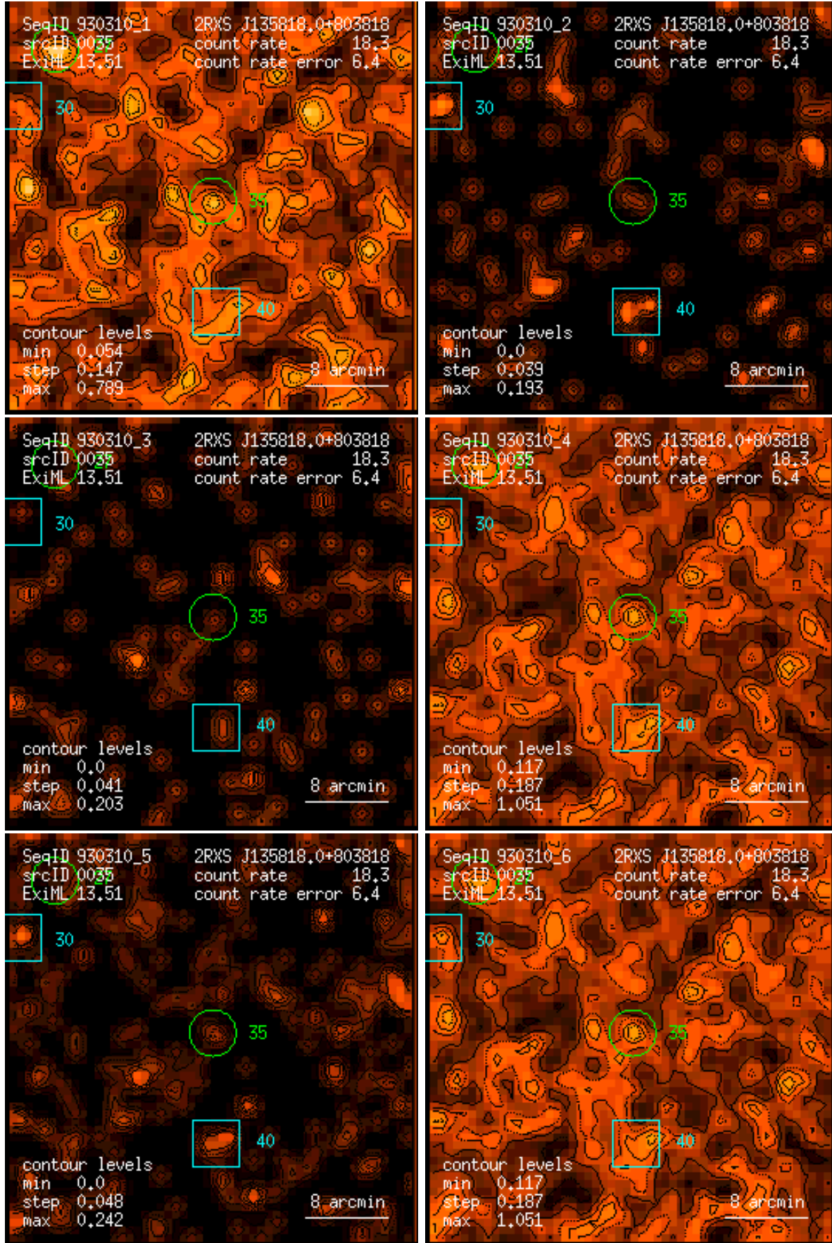
Figure 35: RASS 930310: detection 0035: band rate images, Gaussian filter: (1) PSPC channels 11 – 41, (2) 52 – 90, (3) 91 – 201, (4) 11 – 235, (5) 52 – 201, (6) 11 – 201. Broad band rates in counts/ks. Band rate contour levels in counts/ks/arcmin 2 .
