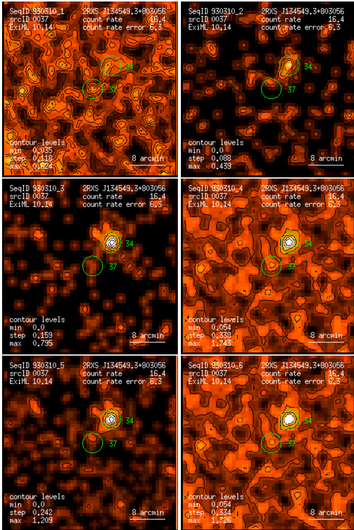
Figure 37: RASS 930310: detection 0037: band rate images, Gaussian filter: (1) PSPC channels 11 – 41, (2) 52 – 90, (3) 91 – 201, (4) 11 – 235, (5) 52 – 201, (6) 11 – 201. Broad band rates in counts/ks. Band rate contour levels in counts/ks/arcmin 2 .
