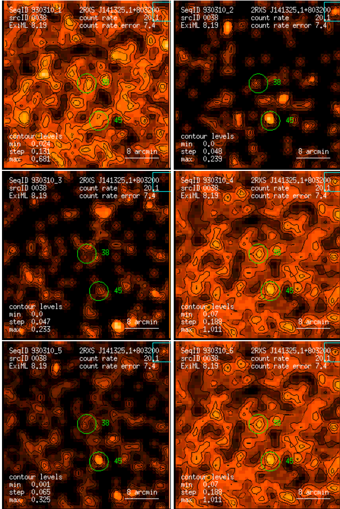
Figure 38: RASS 930310: detection 0038: band rate images, Gaussian filter: (1) PSPC channels 11 – 41, (2) 52 – 90, (3) 91 – 201, (4) 11 – 235, (5) 52 – 201, (6) 11 – 201. Broad band rates in counts/ks. Band rate contour levels in counts/ks/arcmin 2 .
