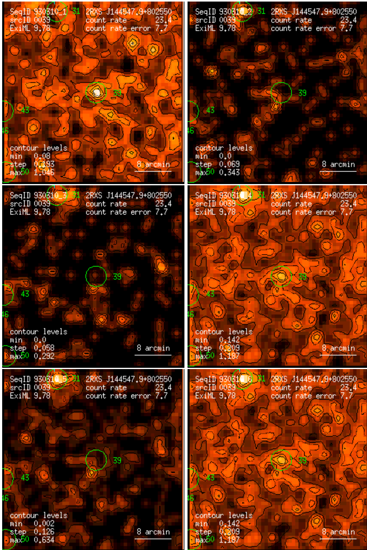
Figure 39: RASS 930310: detection 0039: band rate images, Gaussian filter: (1) PSPC channels 11 – 41, (2) 52 – 90, (3) 91 – 201, (4) 11 – 235, (5) 52 – 201, (6) 11 – 201. Broad band rates in counts/ks. Band rate contour levels in counts/ks/arcmin 2 .
