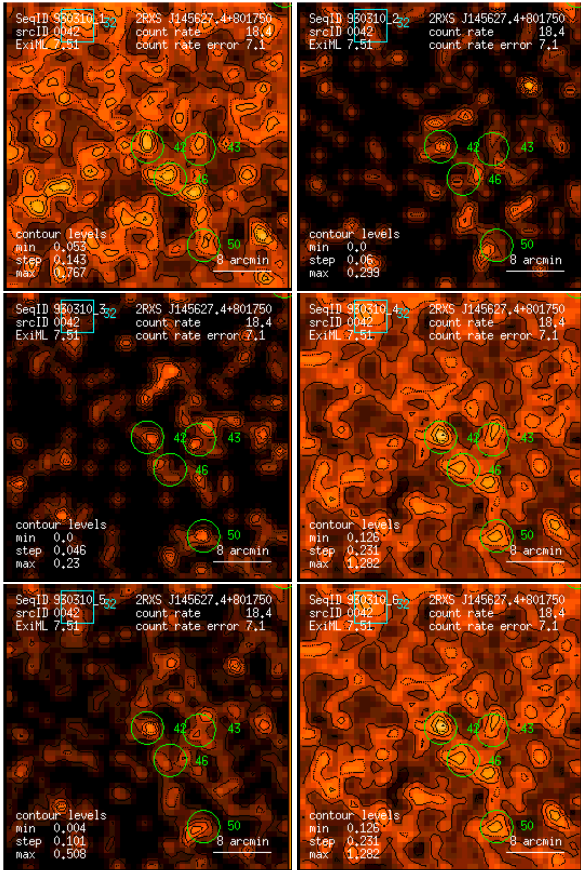
Figure 42: RASS 930310: detection 0042: band rate images, Gaussian filter: (1) PSPC channels 11 – 41, (2) 52 – 90, (3) 91 – 201, (4) 11 – 235, (5) 52 – 201, (6) 11 – 201. Broad band rates in counts/ks. Band rate contour levels in counts/ks/arcmin 2 .
