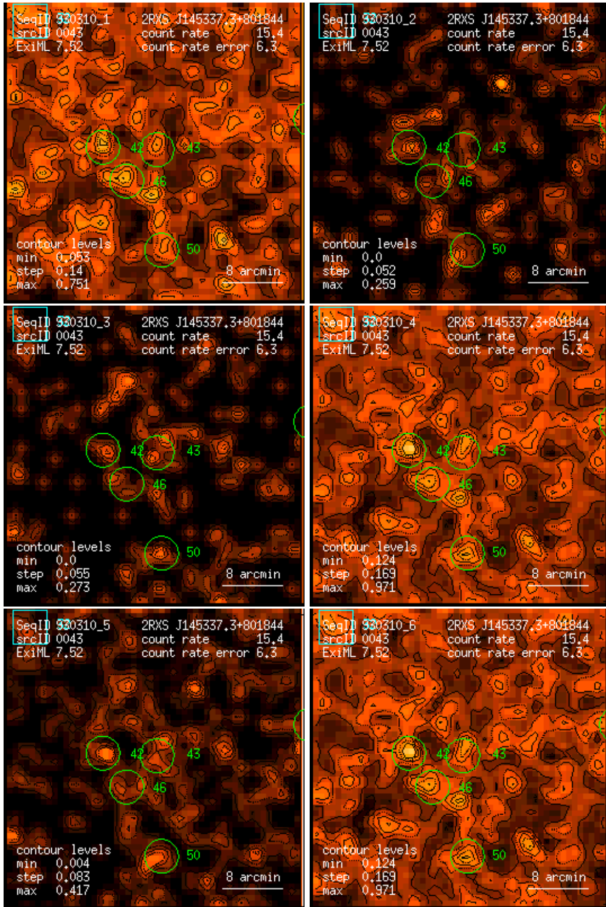
Figure 43: RASS 930310: detection 0043: band rate images, Gaussian filter: (1) PSPC channels 11 – 41, (2) 52 – 90, (3) 91 – 201, (4) 11 – 235, (5) 52 – 201, (6) 11 – 201. Broad band rates in counts/ks. Band rate contour levels in counts/ks/arcmin 2 .
