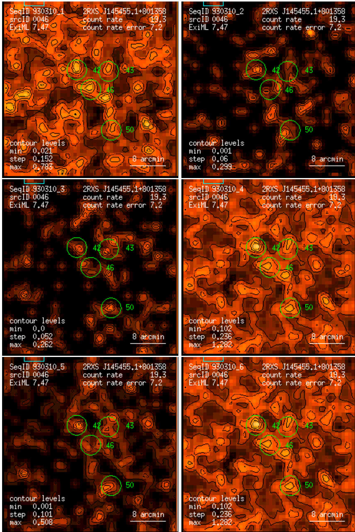
Figure 46: RASS 930310: detection 0046: band rate images, Gaussian filter: (1) PSPC channels 11 – 41, (2) 52 – 90, (3) 91 – 201, (4) 11 – 235, (5) 52 – 201, (6) 11 – 201. Broad band rates in counts/ks. Band rate contour levels in counts/ks/arcmin 2 .
