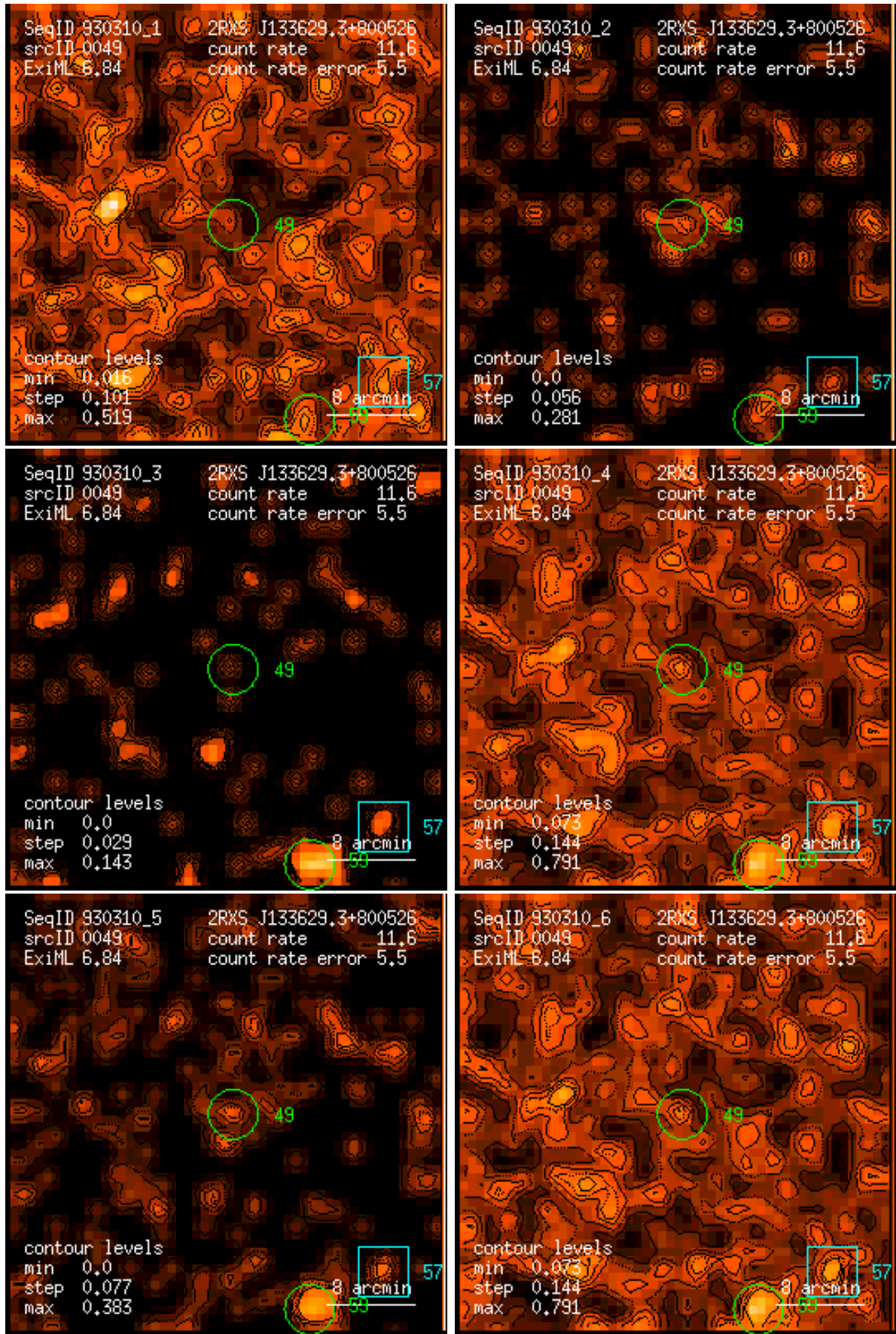
Figure 49: RASS 930310: detection 0049: band rate images, Gaussian filter: (1) PSPC channels 11 – 41, (2) 52 – 90, (3) 91 – 201, (4) 11 – 235, (5) 52 – 201, (6) 11 – 201. Broad band rates in counts/ks. Band rate contour levels in counts/ks/arcmin 2 .
