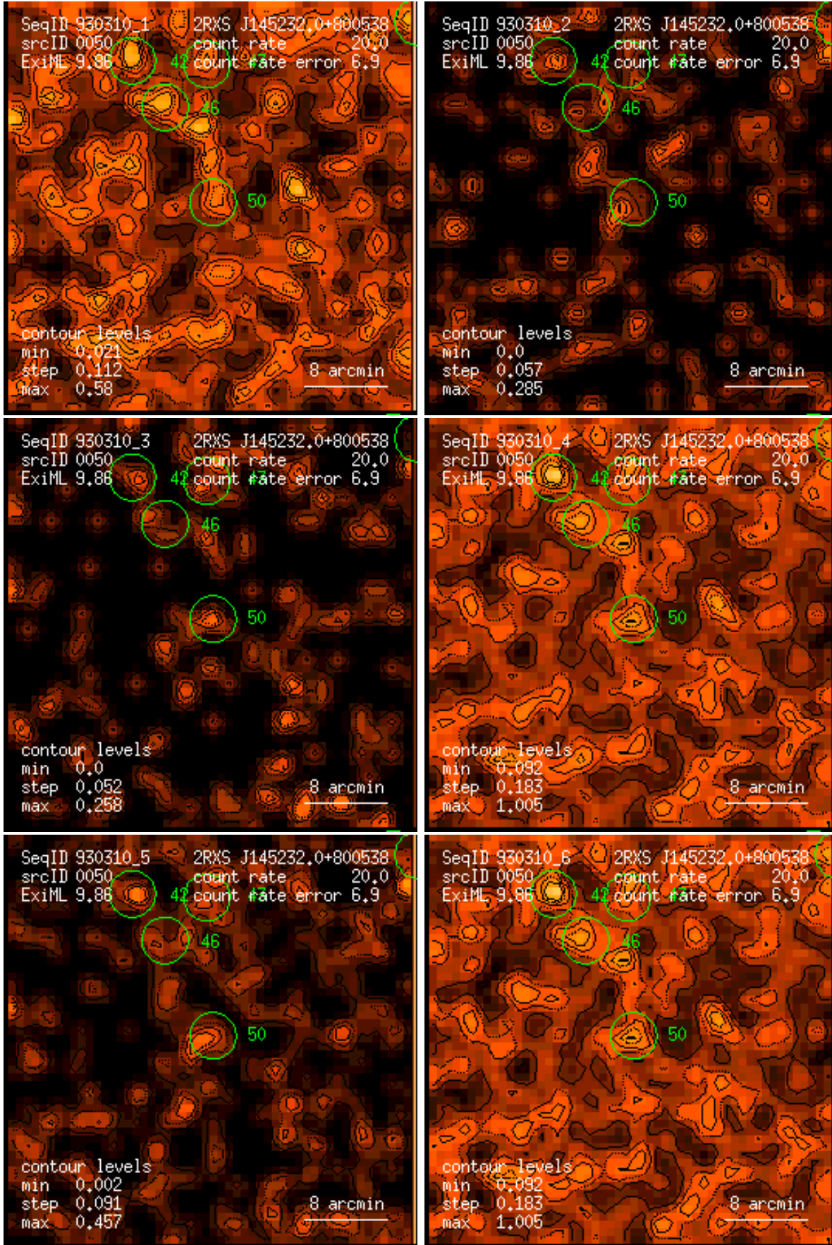
Figure 50: RASS 930310: detection 0050: band rate images, Gaussian filter: (1) PSPC channels 11 – 41, (2) 52 – 90, (3) 91 – 201, (4) 11 – 235, (5) 52 – 201, (6) 11 – 201. Broad band rates in counts/ks. Band rate contour levels in counts/ks/arcmin 2 .
