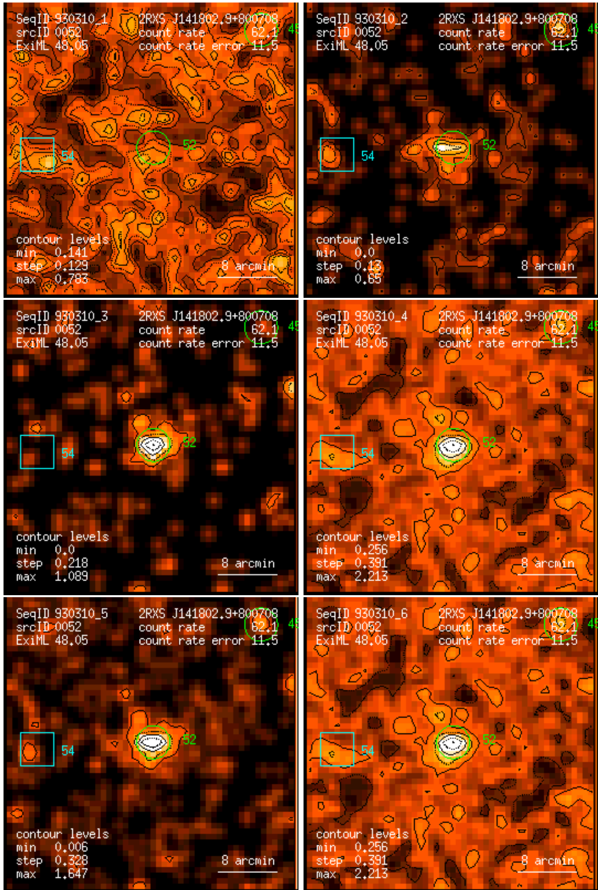
Figure 52: RASS 930310: detection 0052: band rate images, Gaussian filter: (1) PSPC channels 11 – 41, (2) 52 – 90, (3) 91 – 201, (4) 11 – 235, (5) 52 – 201, (6) 11 – 201. Broad band rates in counts/ks. Band rate contour levels in counts/ks/arcmin 2 .
