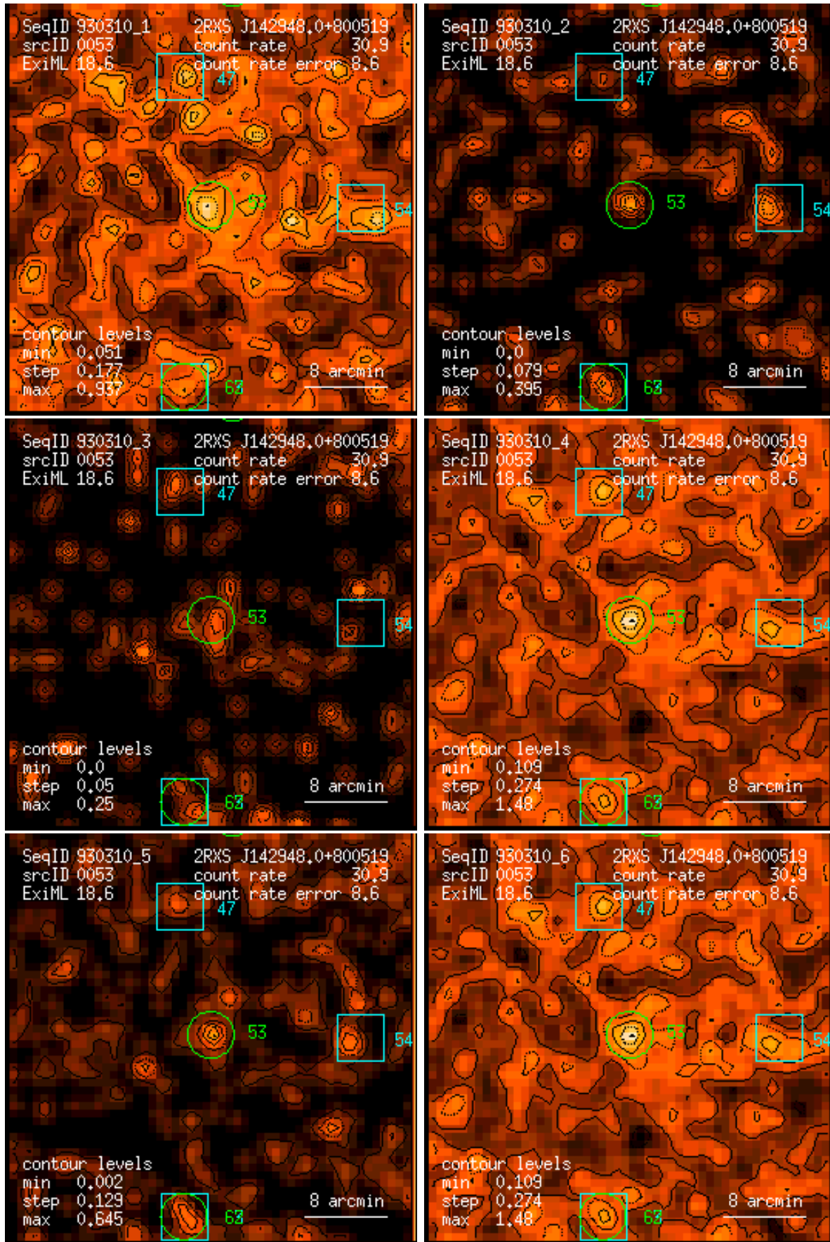
Figure 53: RASS 930310: detection 0053: band rate images, Gaussian filter: (1) PSPC channels 11 – 41, (2) 52 – 90, (3) 91 – 201, (4) 11 – 235, (5) 52 – 201, (6) 11 – 201. Broad band rates in counts/ks. Band rate contour levels in counts/ks/arcmin 2 .
