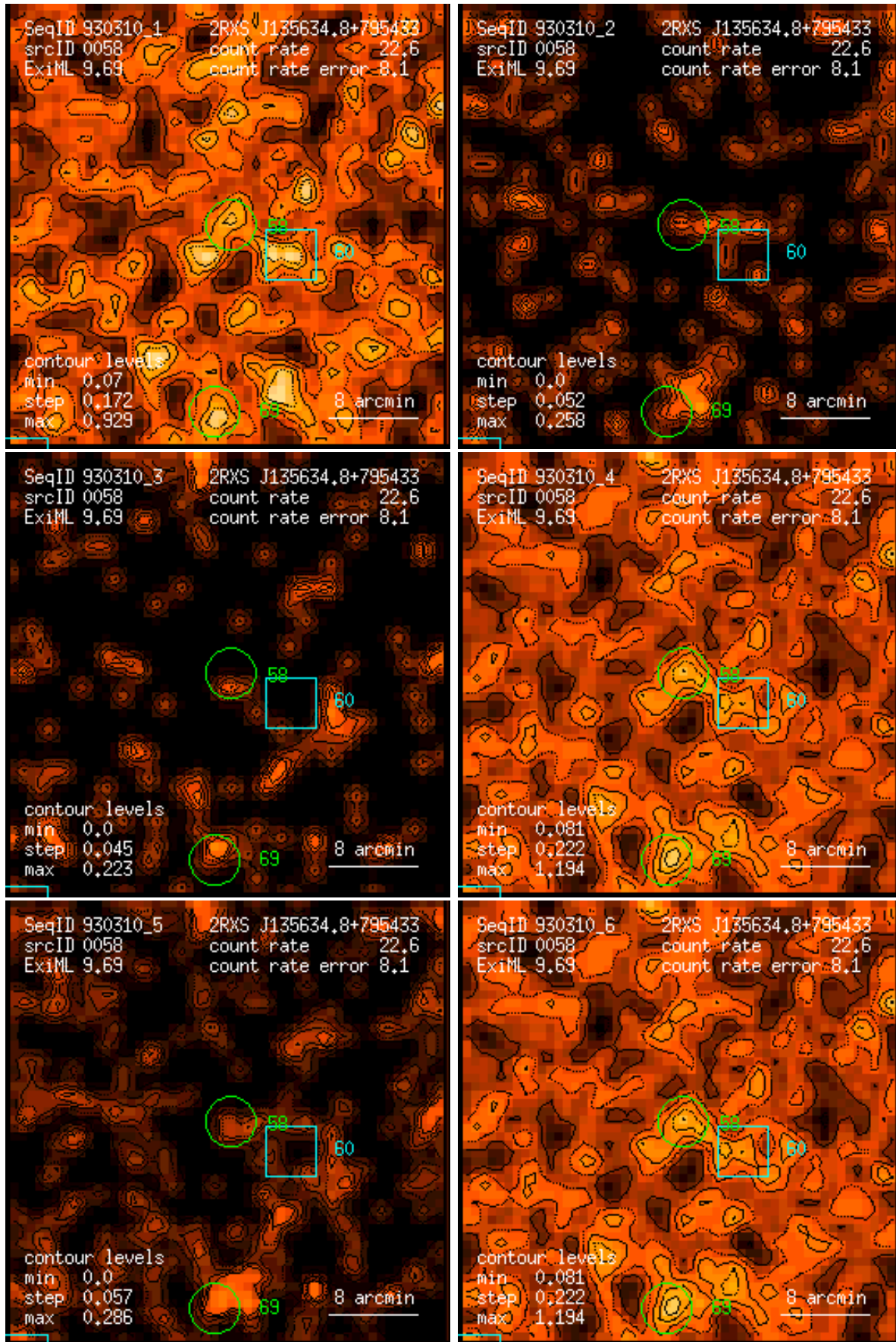
Figure 58: RASS 930310: detection 0058: band rate images, Gaussian filter: (1) PSPC channels 11 – 41, (2) 52 – 90, (3) 91 – 201, (4) 11 – 235, (5) 52 – 201, (6) 11 – 201. Broad band rates in counts/ks. Band rate contour levels in counts/ks/arcmin 2 .
