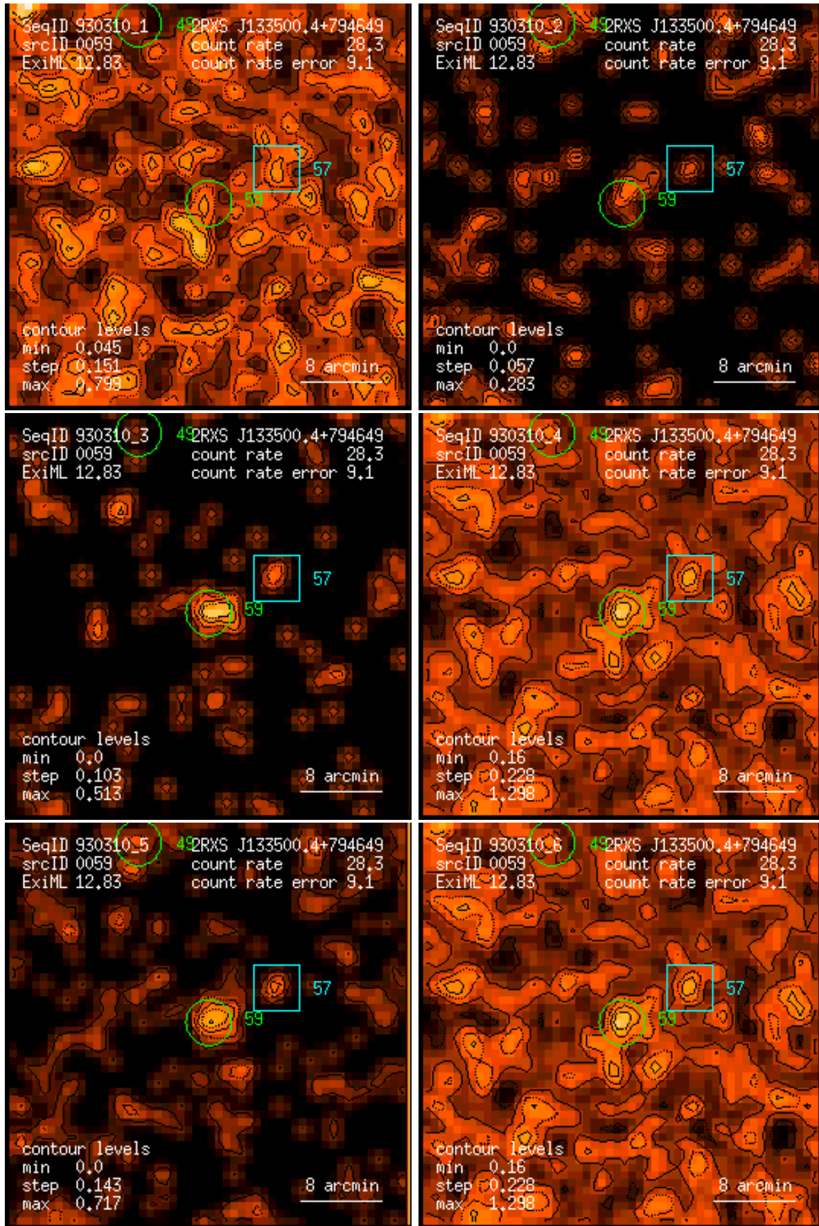
Figure 59: RASS 930310: detection 0059: band rate images, Gaussian filter: (1) PSPC channels 11 – 41, (2) 52 – 90, (3) 91 – 201, (4) 11 – 235, (5) 52 – 201, (6) 11 – 201. Broad band rates in counts/ks. Band rate contour levels in counts/ks/arcmin 2 .
