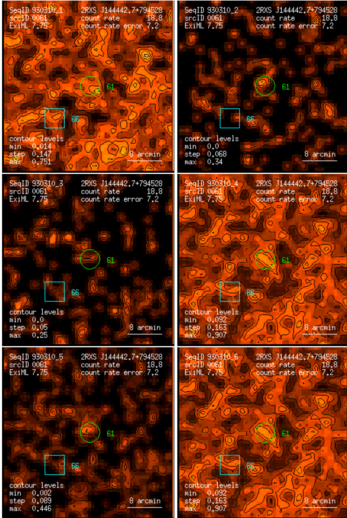
Figure 61: RASS 930310: detection 0061: band rate images, Gaussian filter: (1) PSPC channels 11 – 41, (2) 52 – 90, (3) 91 – 201, (4) 11 – 235, (5) 52 – 201, (6) 11 – 201. Broad band rates in counts/ks. Band rate contour levels in counts/ks/arcmin 2 .
