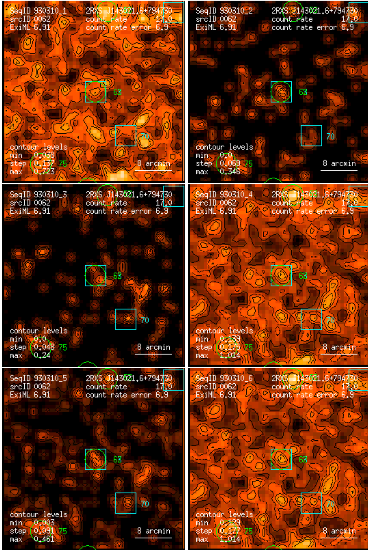
Figure 62: RASS 930310: detection 0062: band rate images, Gaussian filter: (1) PSPC channels 11 – 41, (2) 52 – 90, (3) 91 – 201, (4) 11 – 235, (5) 52 – 201, (6) 11 – 201. Broad band rates in counts/ks. Band rate contour levels in counts/ks/arcmin 2 .
