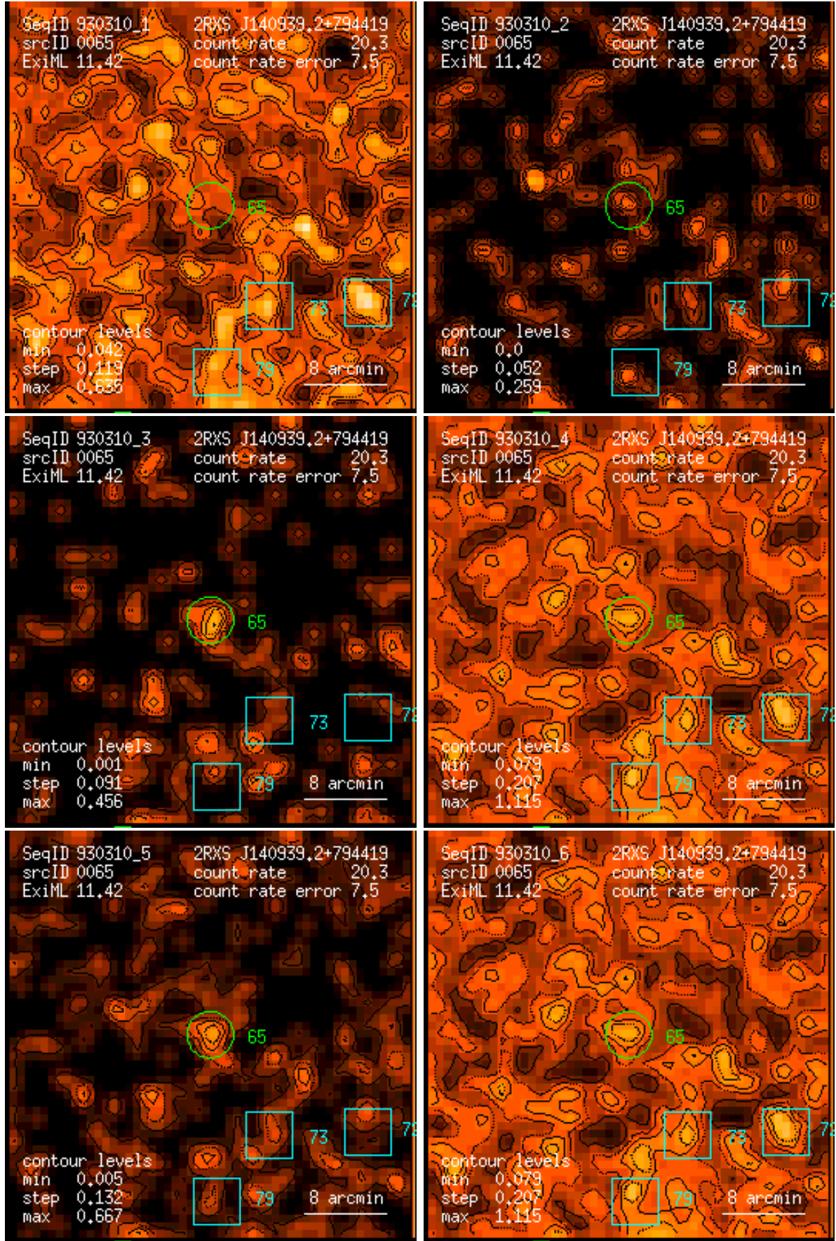
Figure 65: RASS 930310: detection 0065: band rate images, Gaussian filter: (1) PSPC channels 11 – 41, (2) 52 – 90, (3) 91 – 201, (4) 11 – 235, (5) 52 – 201, (6) 11 – 201. Broad band rates in counts/ks. Band rate contour levels in counts/ks/arcmin 2 .
