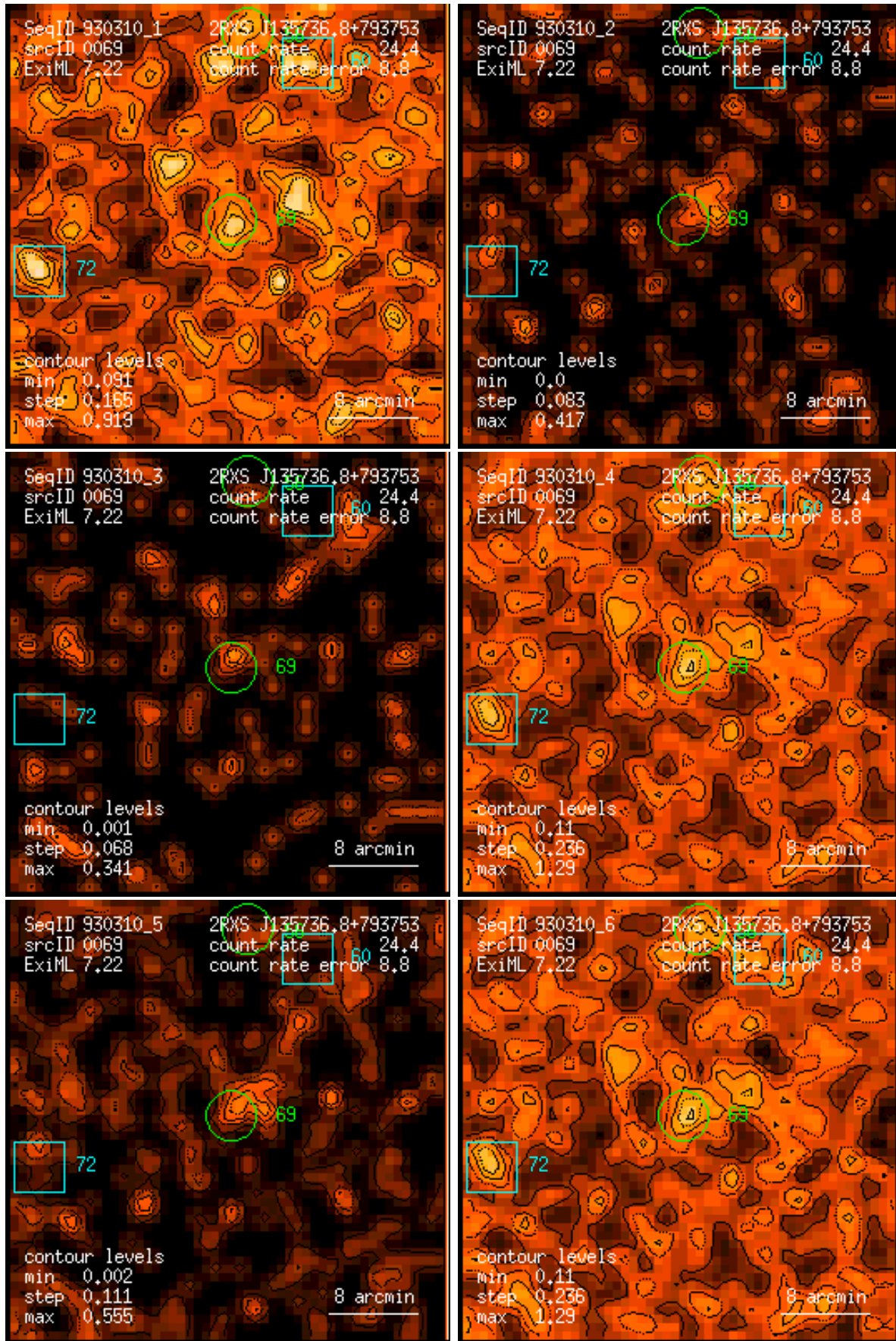
Figure 69: RASS 930310: detection 0069: band rate images, Gaussian filter: (1) PSPC channels 11 – 41, (2) 52 – 90, (3) 91 – 201, (4) 11 – 235, (5) 52 – 201, (6) 11 – 201. Broad band rates in counts/ks. Band rate contour levels in counts/ks/arcmin 2 .
