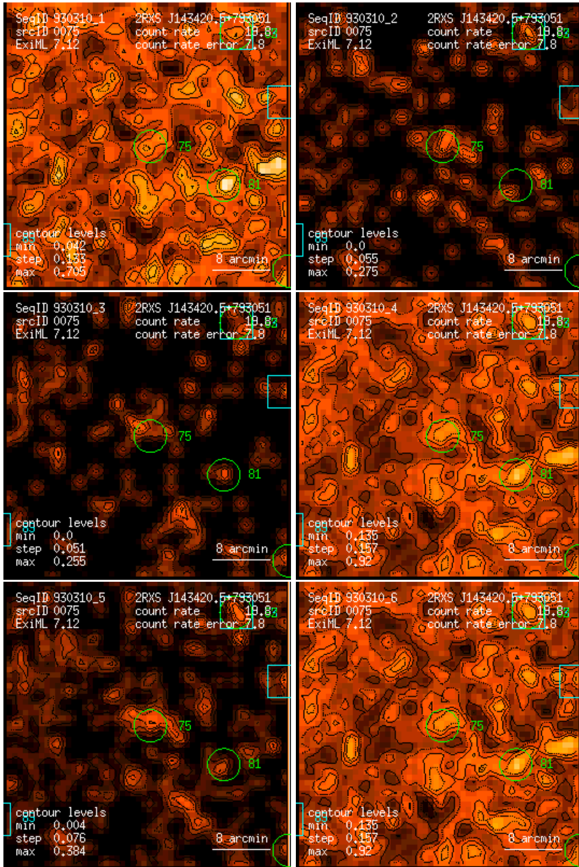
Figure 75: RASS 930310: detection 0075: band rate images, Gaussian filter: (1) PSPC channels 11 – 41, (2) 52 – 90, (3) 91 – 201, (4) 11 – 235, (5) 52 – 201, (6) 11 – 201. Broad band rates in counts/ks. Band rate contour levels in counts/ks/arcmin 2 .
