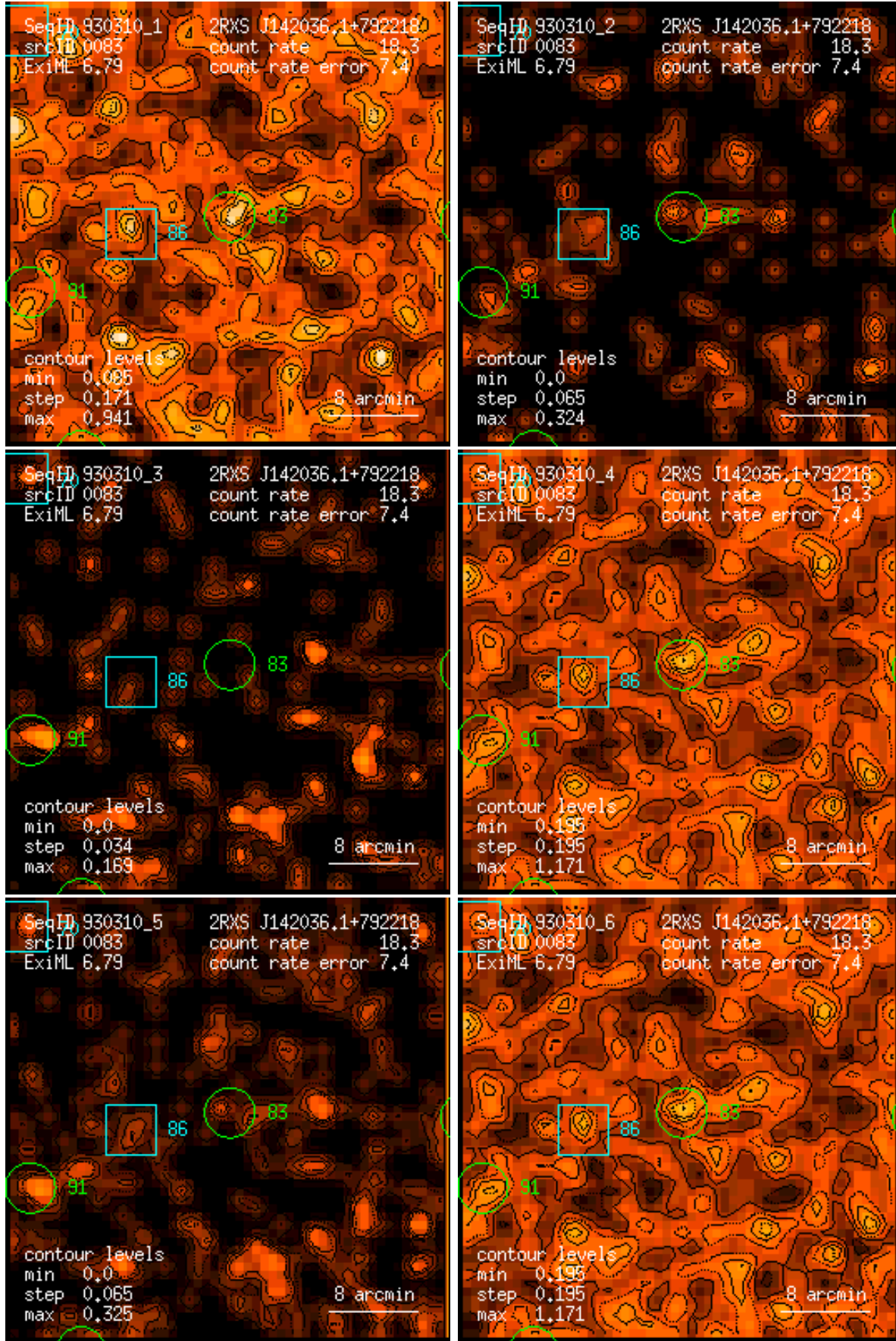
Figure 83: RASS 930310: detection 0083: band rate images, Gaussian filter: (1) PSPC channels 11 – 41, (2) 52 – 90, (3) 91 – 201, (4) 11 – 235, (5) 52 – 201, (6) 11 – 201. Broad band rates in counts/ks. Band rate contour levels in counts/ks/arcmin 2 .
