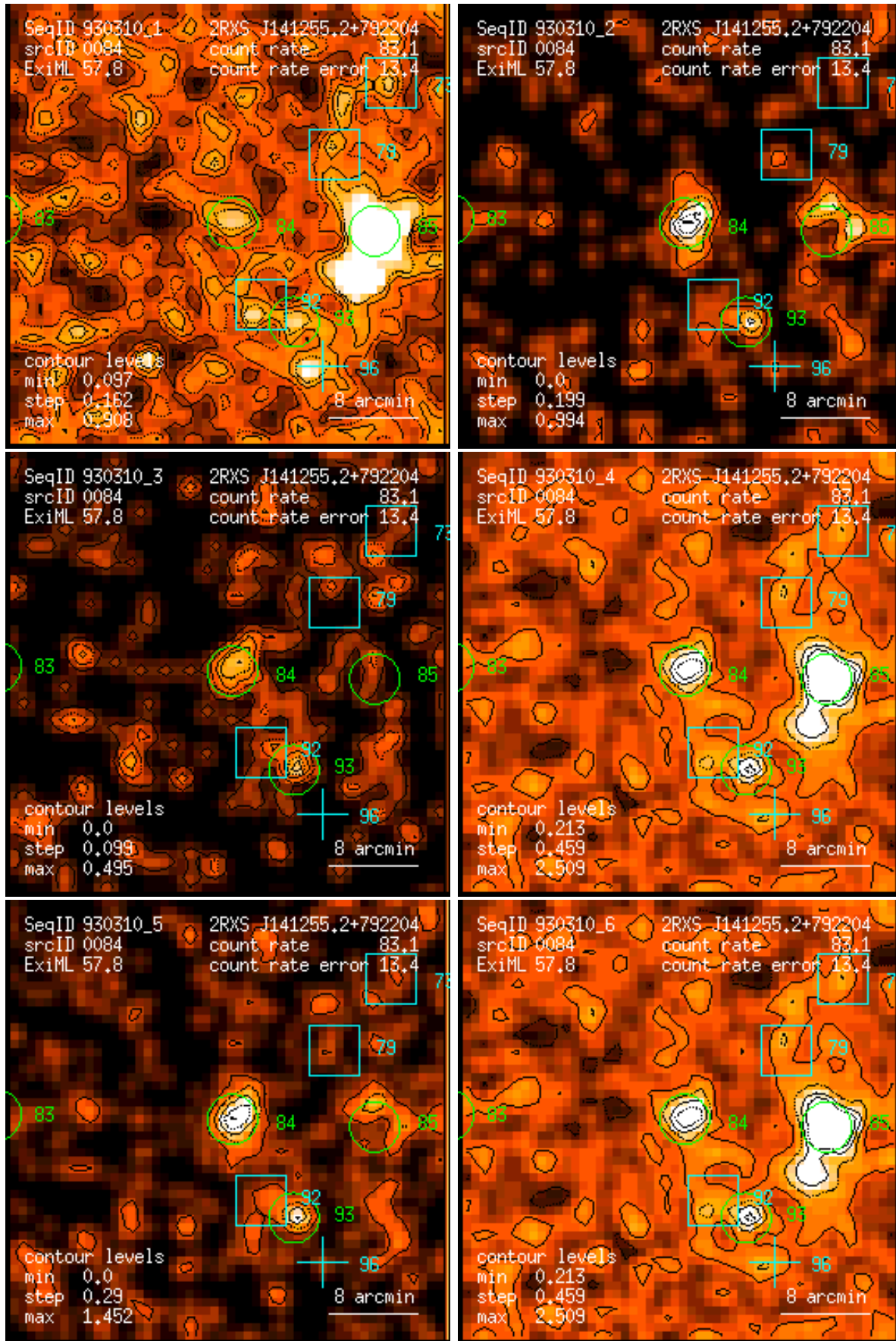
Figure 84: RASS 930310: detection 0084: band rate images, Gaussian filter: (1) PSPC channels 11 – 41, (2) 52 – 90, (3) 91 – 201, (4) 11 – 235, (5) 52 – 201, (6) 11 – 201. Broad band rates in counts/ks. Band rate contour levels in counts/ks/arcmin 2 .
