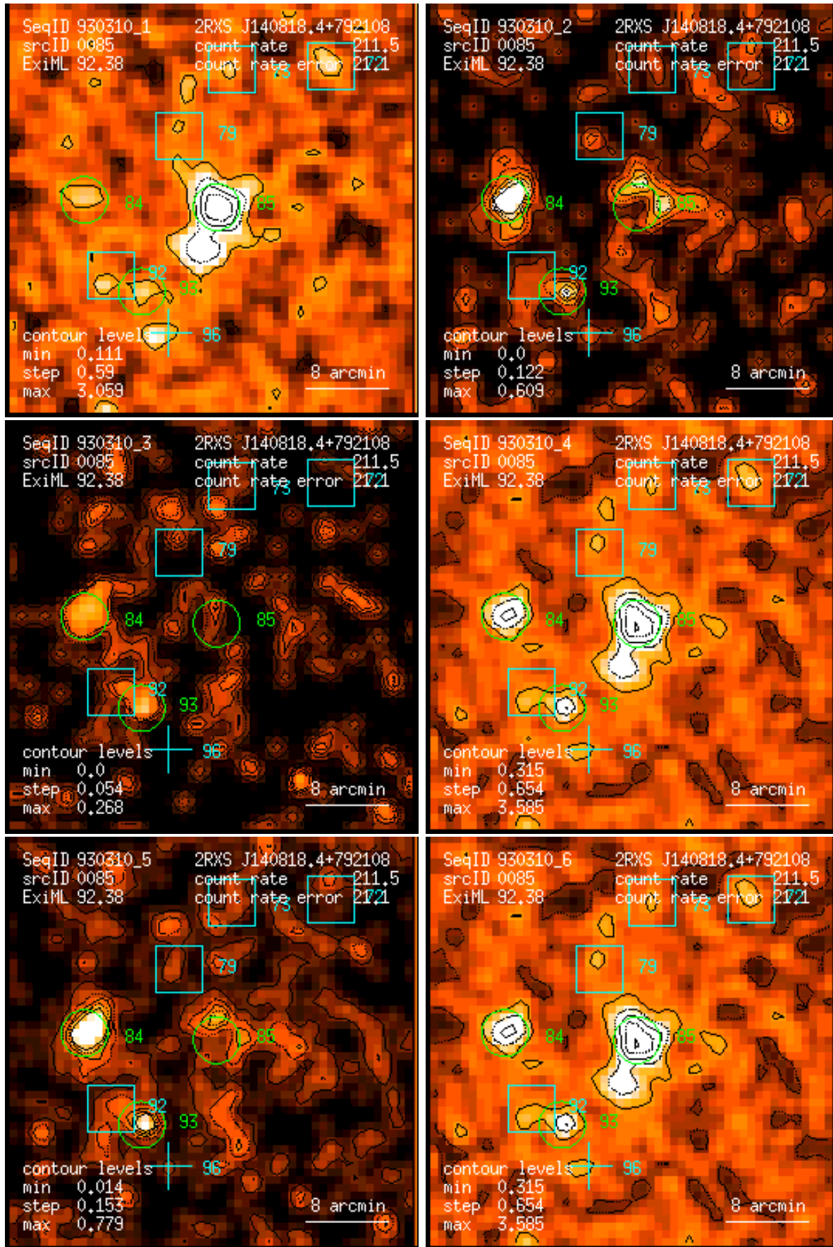
Figure 85: RASS 930310: detection 0085: band rate images, Gaussian filter: (1) PSPC channels 11 – 41, (2) 52 – 90, (3) 91 – 201, (4) 11 – 235, (5) 52 – 201, (6) 11 – 201. Broad band rates in counts/ks. Band rate contour levels in counts/ks/arcmin 2 .
