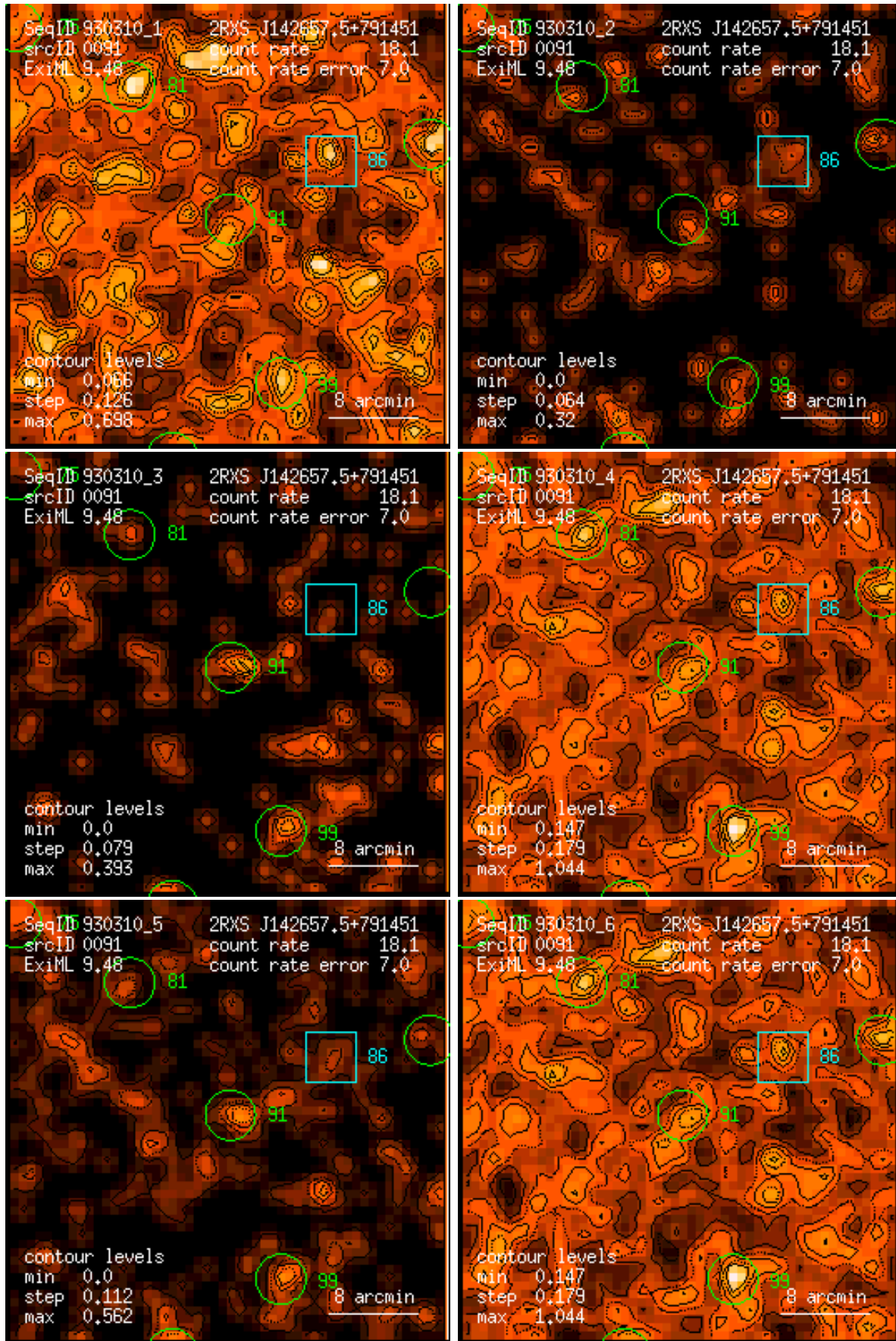
Figure 91: RASS 930310: detection 0091: band rate images, Gaussian filter: (1) PSPC channels 11 – 41, (2) 52 – 90, (3) 91 – 201, (4) 11 – 235, (5) 52 – 201, (6) 11 – 201. Broad band rates in counts/ks. Band rate contour levels in counts/ks/arcmin 2 .
