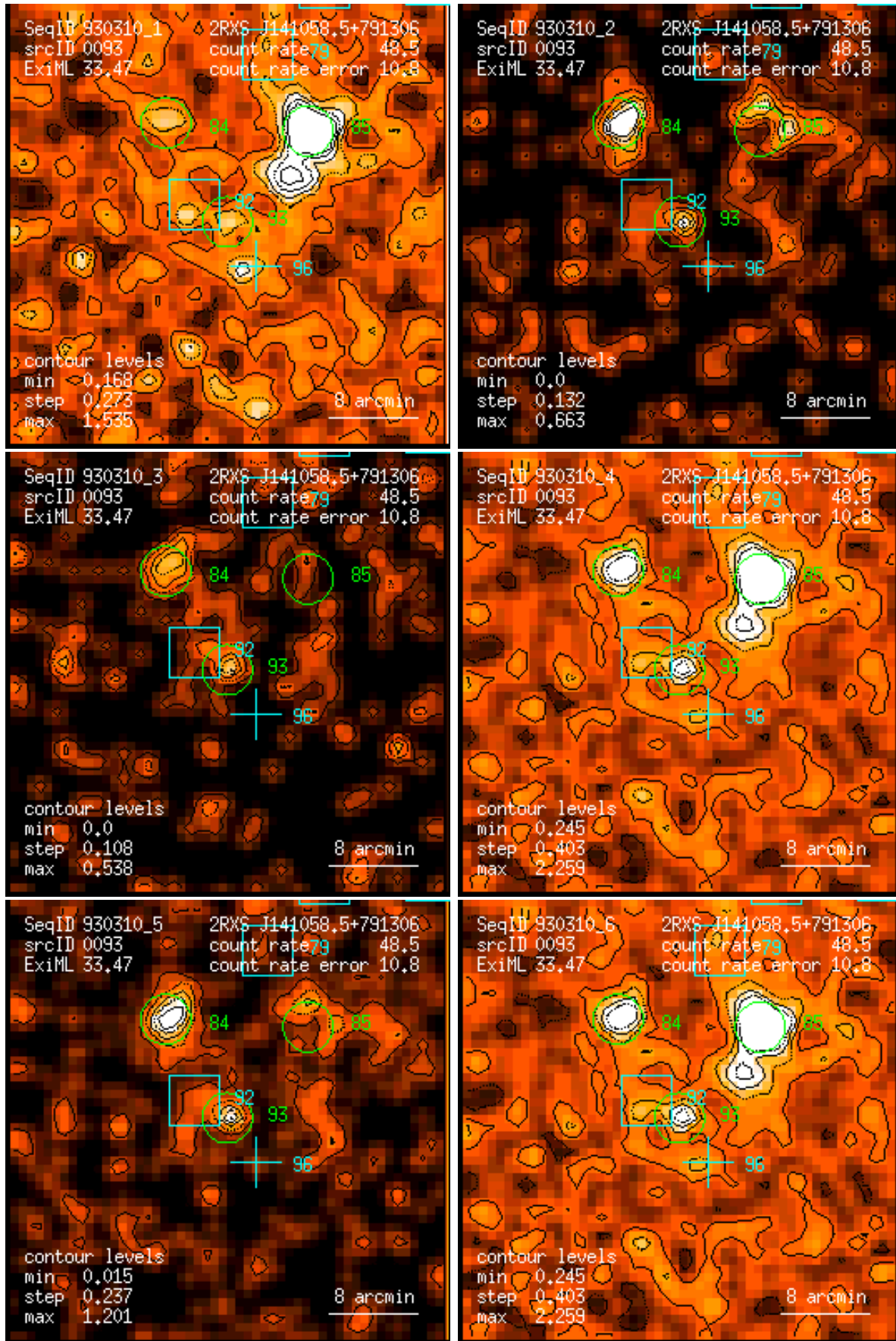
Figure 93: RASS 930310: detection 0093: band rate images, Gaussian filter: (1) PSPC channels 11 – 41, (2) 52 – 90, (3) 91 – 201, (4) 11 – 235, (5) 52 – 201, (6) 11 – 201. Broad band rates in counts/ks. Band rate contour levels in counts/ks/arcmin 2 .
