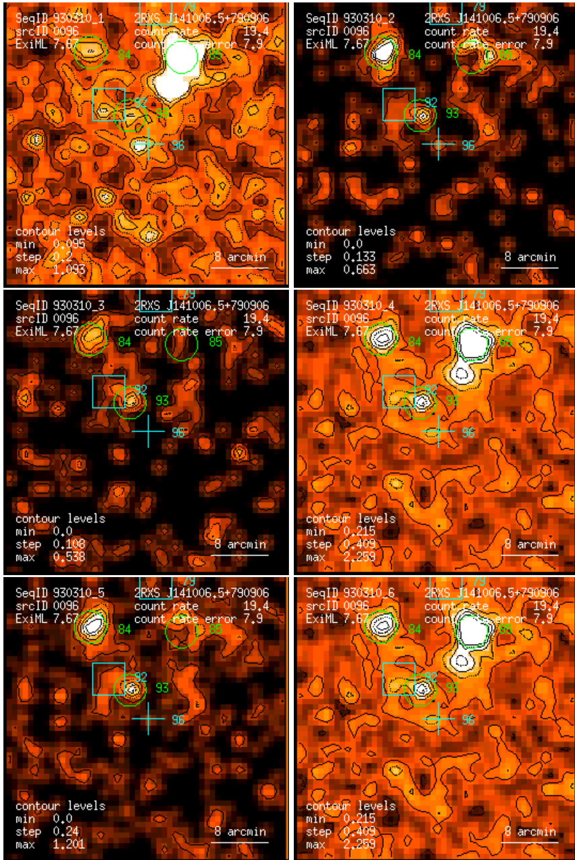
Figure 96: RASS 930310: detection 0096: band rate images, Gaussian filter: (1) PSPC channels 11 – 41, (2) 52 – 90, (3) 91 – 201, (4) 11 – 235, (5) 52 – 201, (6) 11 – 201. Broad band rates in counts/ks. Band rate contour levels in counts/ks/arcmin 2 .
