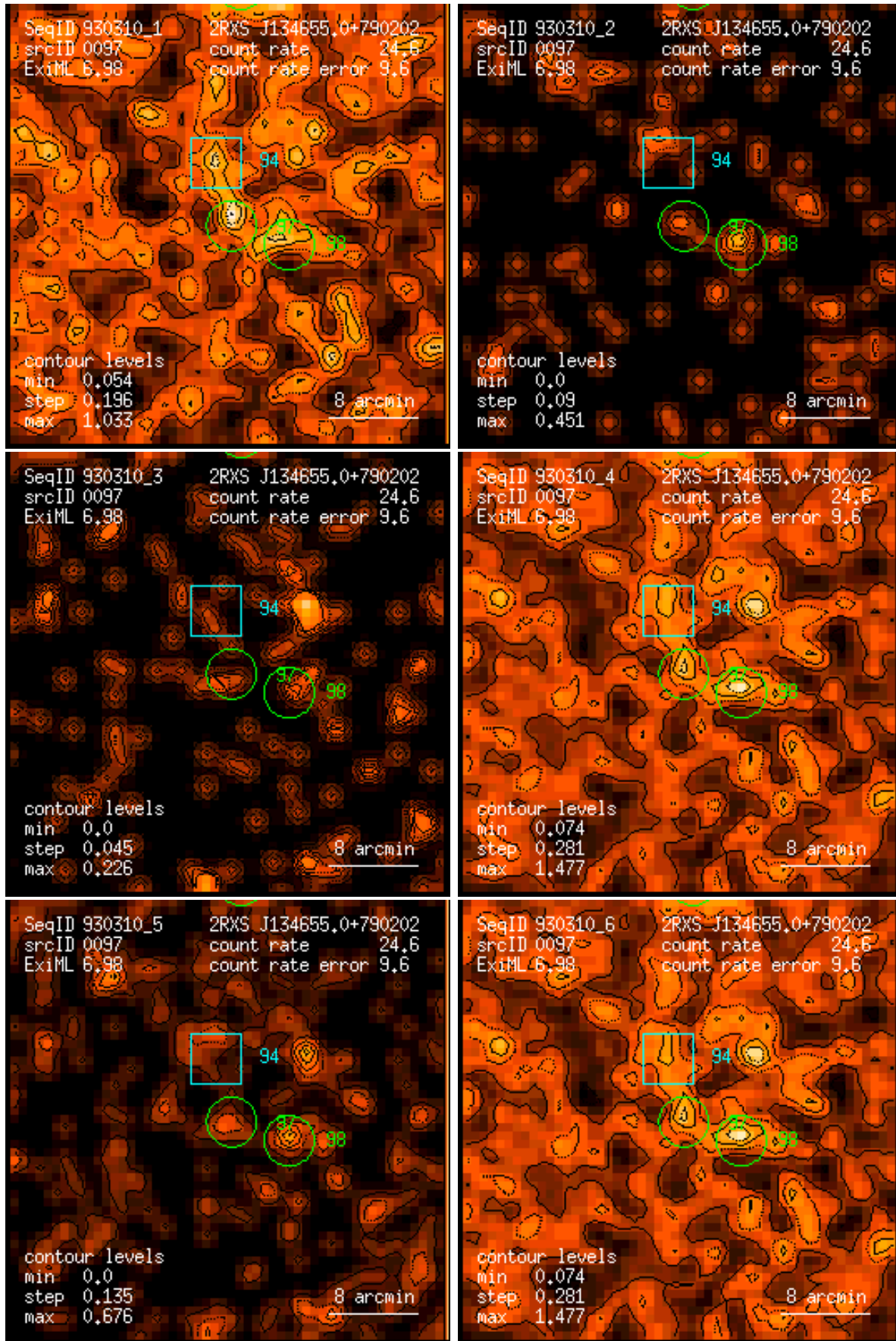
Figure 97: RASS 930310: detection 0097: band rate images, Gaussian filter: (1) PSPC channels 11 – 41, (2) 52 – 90, (3) 91 – 201, (4) 11 – 235, (5) 52 – 201, (6) 11 – 201. Broad band rates in counts/ks. Band rate contour levels in counts/ks/arcmin 2 .
