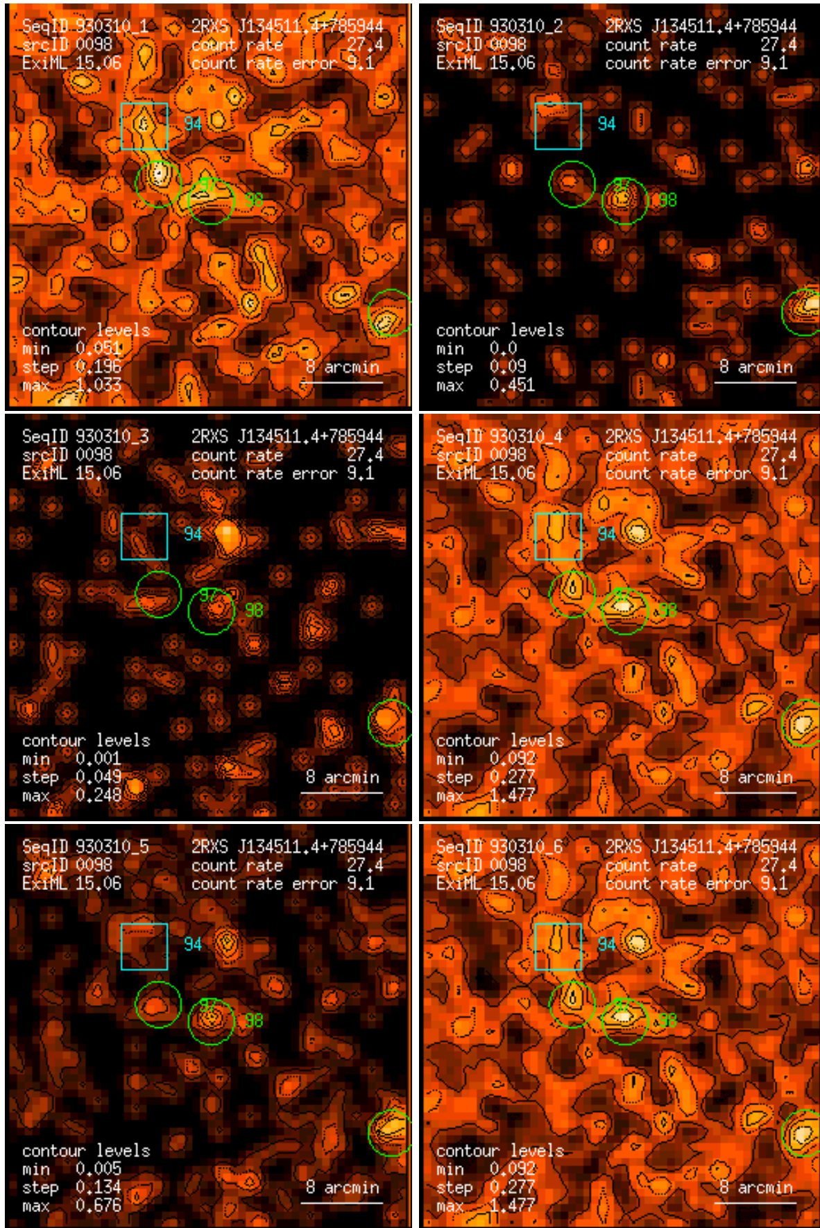
Figure 98: RASS 930310: detection 0098: band rate images, Gaussian filter: (1) PSPC channels 11 – 41, (2) 52 – 90, (3) 91 – 201, (4) 11 – 235, (5) 52 – 201, (6) 11 – 201. Broad band rates in counts/ks. Band rate contour levels in counts/ks/arcmin 2 .
