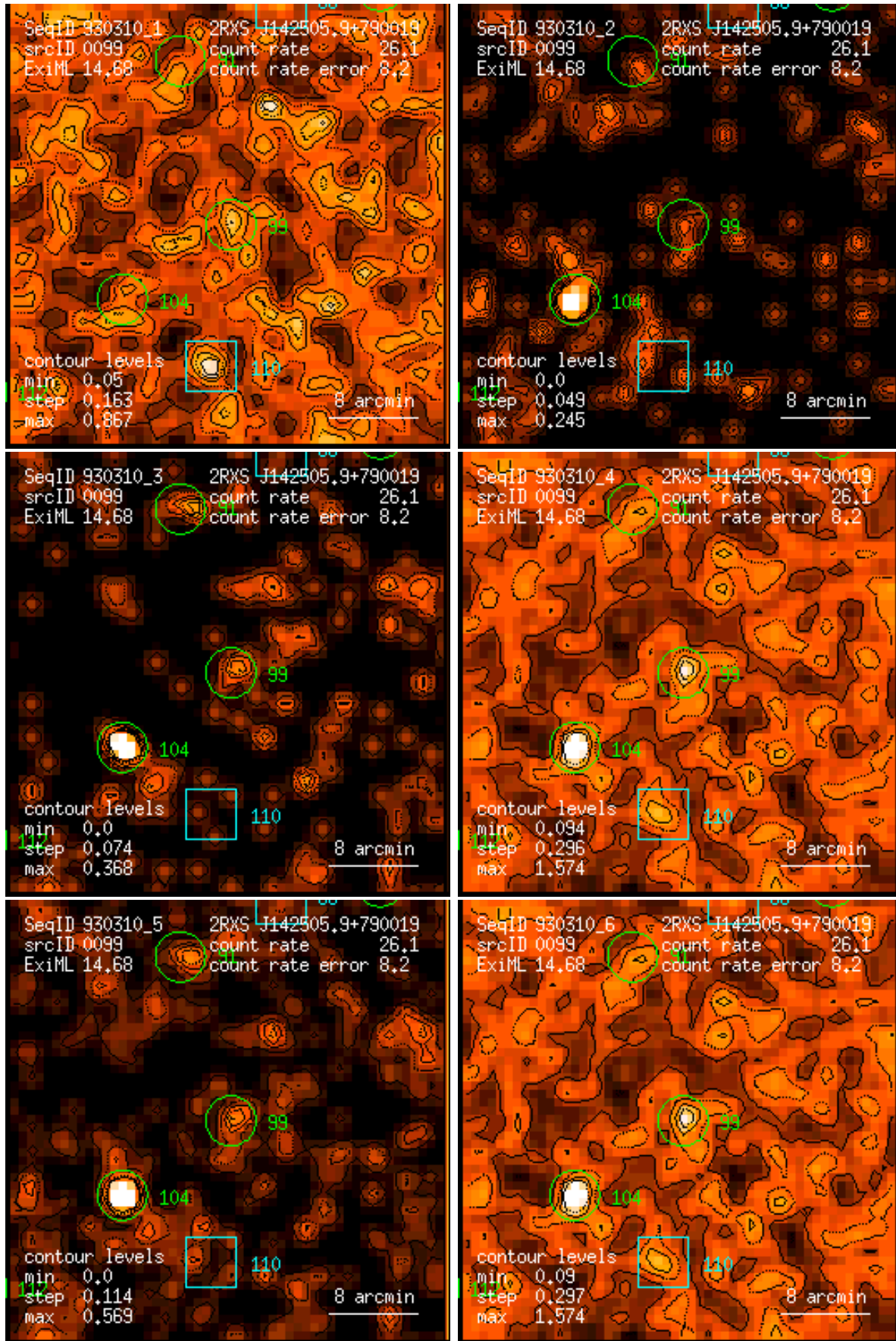
Figure 99: RASS 930310: detection 0099: band rate images, Gaussian filter: (1) PSPC channels 11 – 41, (2) 52 – 90, (3) 91 – 201, (4) 11 – 235, (5) 52 – 201, (6) 11 – 201. Broad band rates in counts/ks. Band rate contour levels in counts/ks/arcmin 2 .
