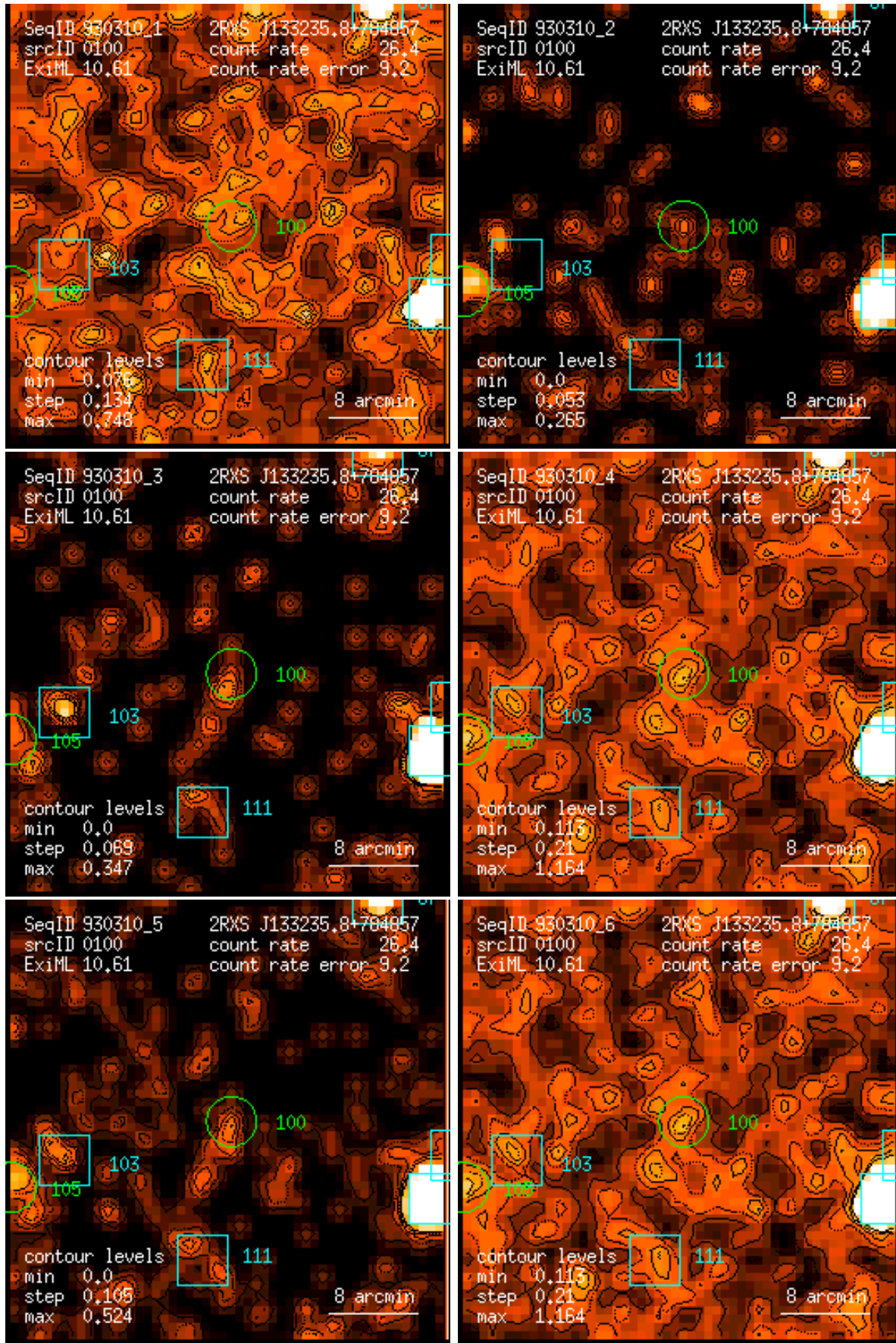
Figure 100: RASS 930310: detection 0100: band rate images, Gaussian filter: (1) PSPC channels 11 – 41, (2) 52 – 90, (3) 91 – 201, (4) 11 – 235, (5) 52 – 201, (6) 11 – 201. Broad band rates in counts/ks. Band rate contour levels in counts/ks/arcmin 2 .
