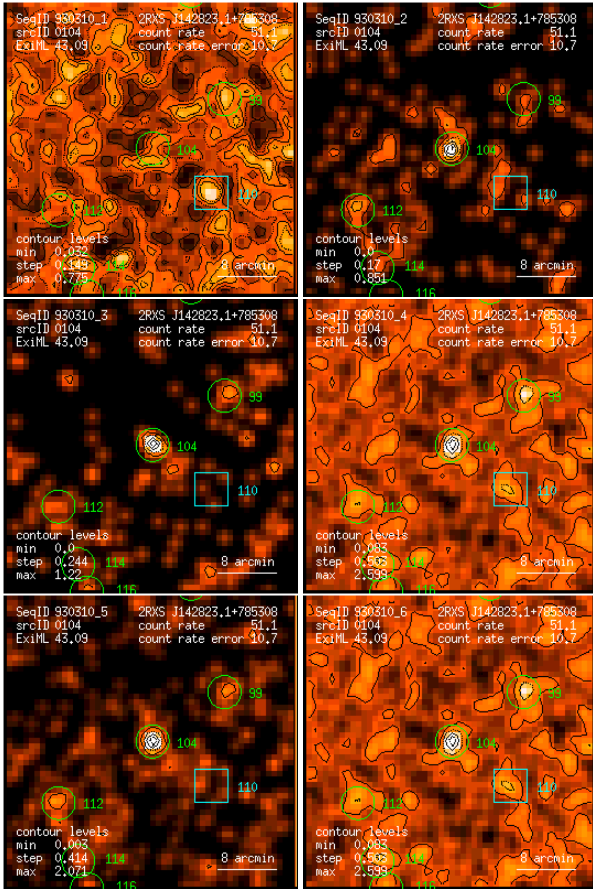
Figure 104: RASS 930310: detection 0104: band rate images, Gaussian filter: (1) PSPC channels 11 – 41, (2) 52 – 90, (3) 91 – 201, (4) 11 – 235, (5) 52 – 201, (6) 11 – 201. Broad band rates in counts/ks. Band rate contour levels in counts/ks/arcmin 2 .
